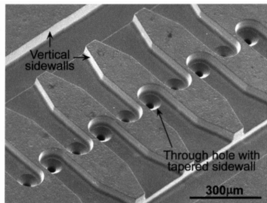
Fig. 5: Arrayed microchannels formed by the sequential application of three different electrode arrays.
