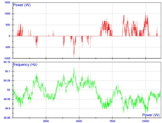
Figure 9: EFR frequency response, frequency (green) and output power (red) against time (seconds)
