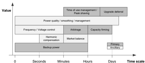
Figure 1: BESS grid services with time scale
