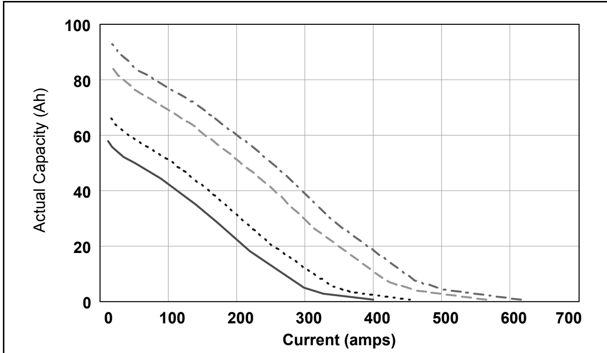
Figure 2 Actual Capacity versus Discharge Current for Four Different NiCd Cell Sizes. (Nominal capacities of cell shown are 58, 67, 85, and 93 amp-hours.)
