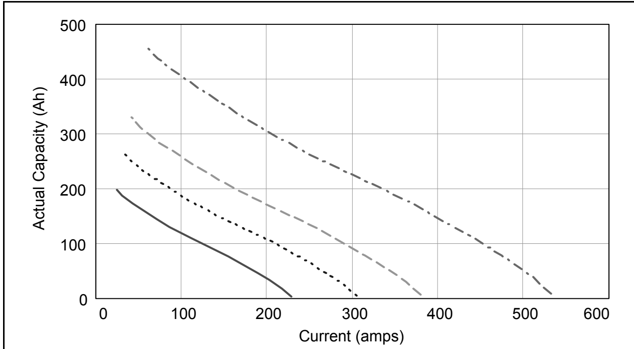
Figure 4 Actual Capacity versus Discharge Current for Four Different VRLA cell sizes. (Nominal capacities of cells shown are 198, 264, 330, and 462 Ah.)
