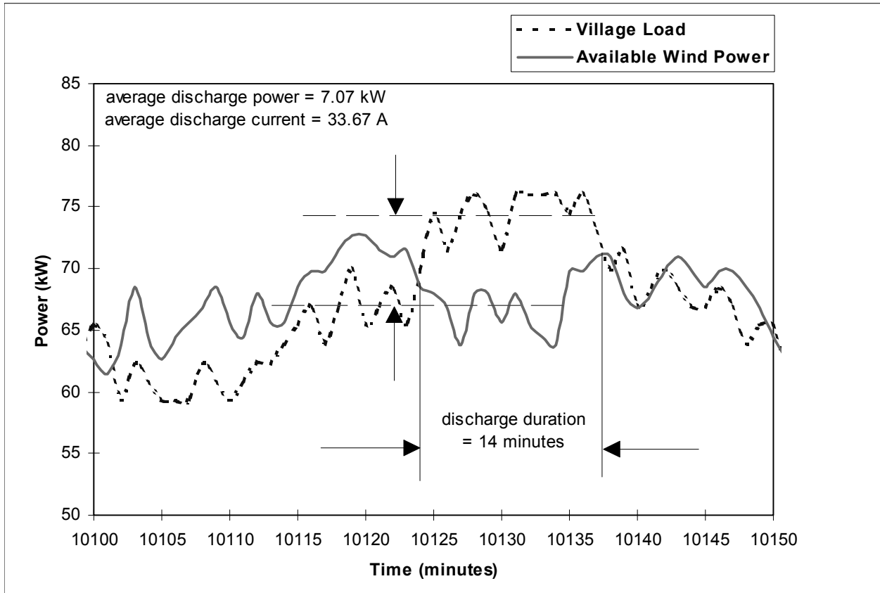
Figure 5 Determination of Current and Duration of Each Discharge Event
