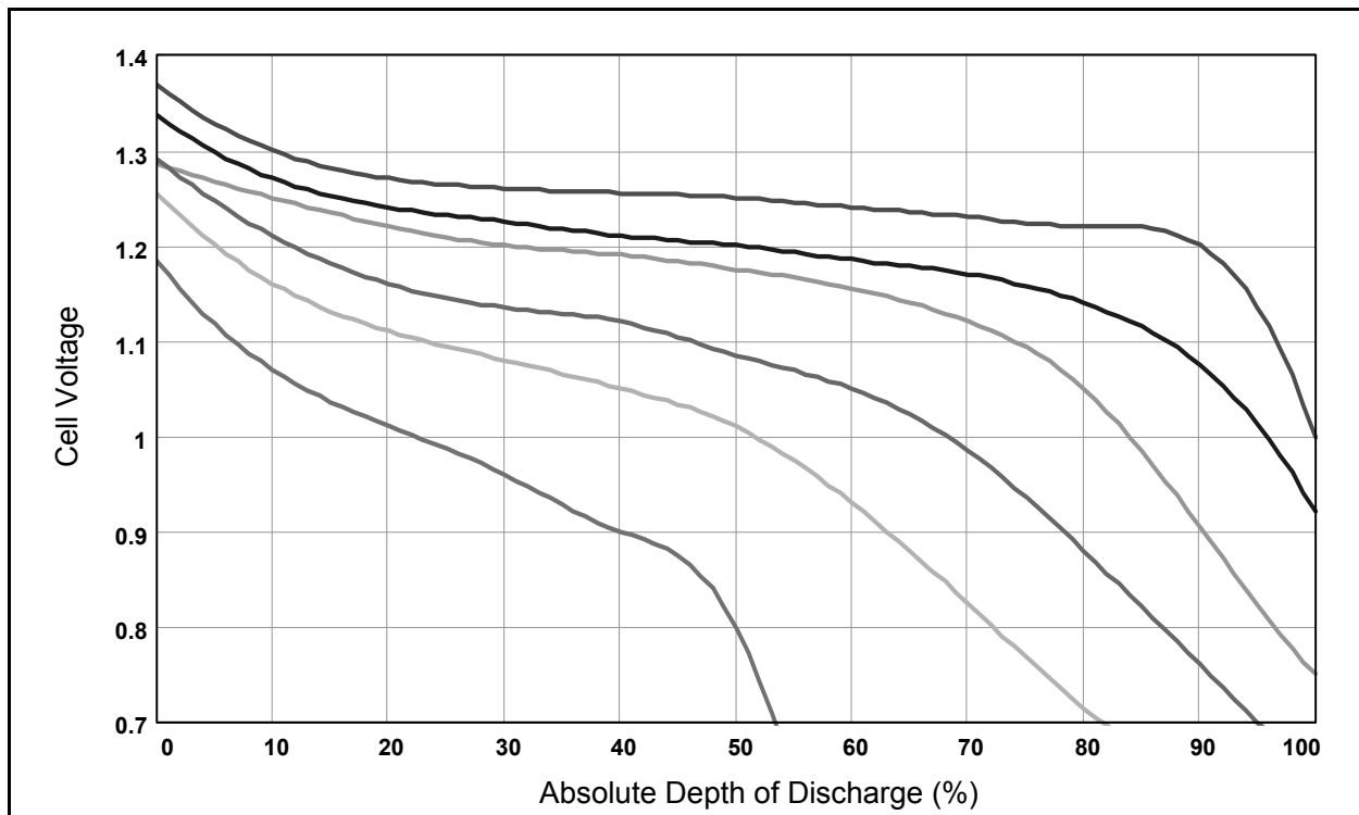
Figure 7 Discharge Voltage versus Depth of Discharge for Various Discharge Currents Based on Manufacturer's Data for Pocket Plate NiCd Cells.
