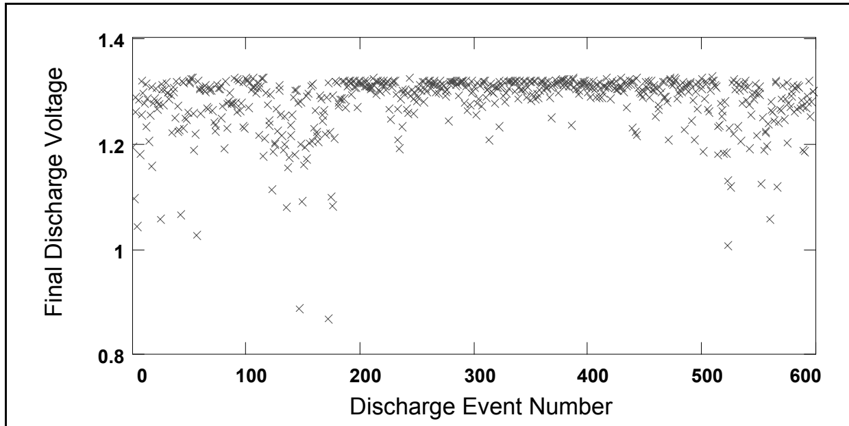
Figure 8 Final Discharge Voltages for each Discharge Event on a 111 Ah NiCd cell.
