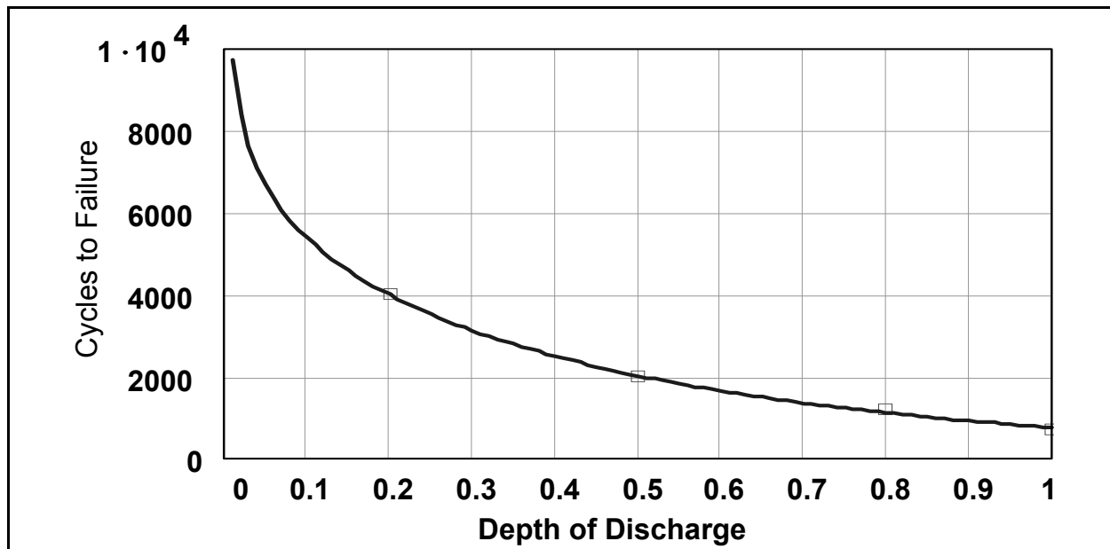
Figure 3 Best fit curve to manufacturer's cycle life data for glass-mat VRLA cells. Equation 3 parameters are u_0=0.19 , u_1=1.69 , and u_2=765 .
