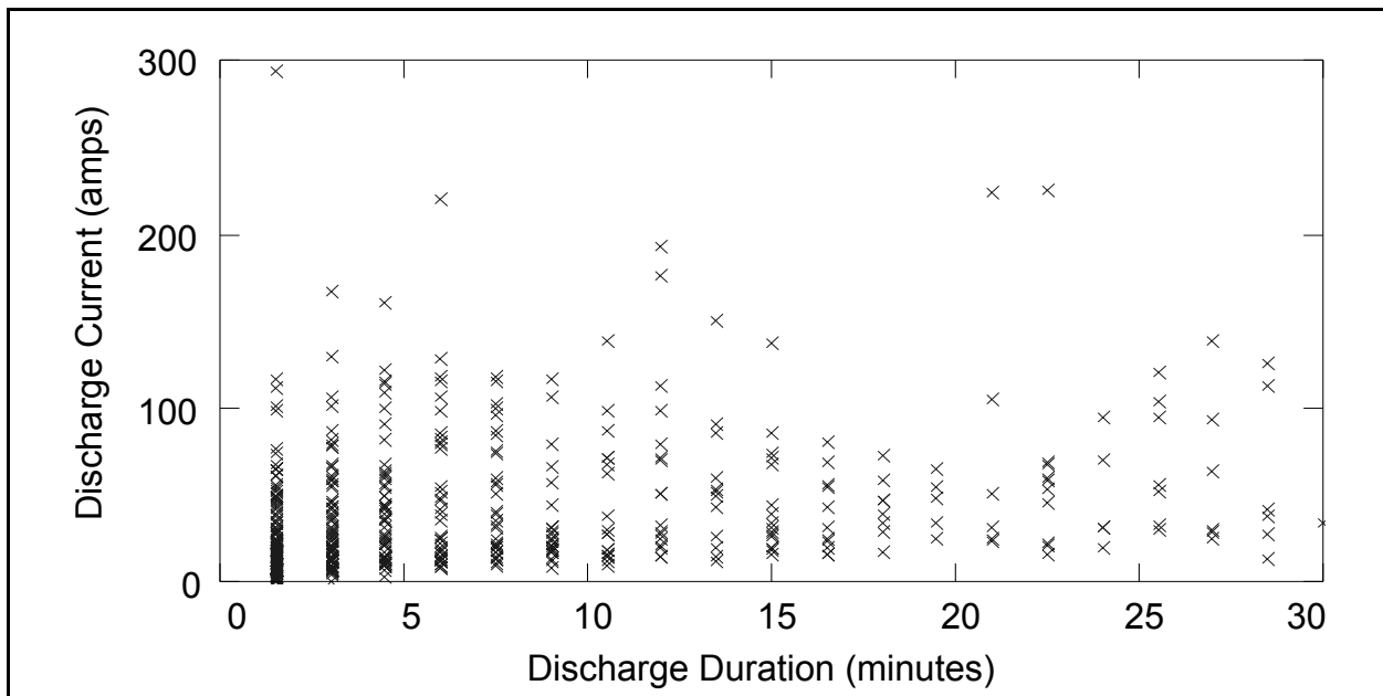
Figure 6 The Complete Data Set of Discharge Events used in the Analysis Example
