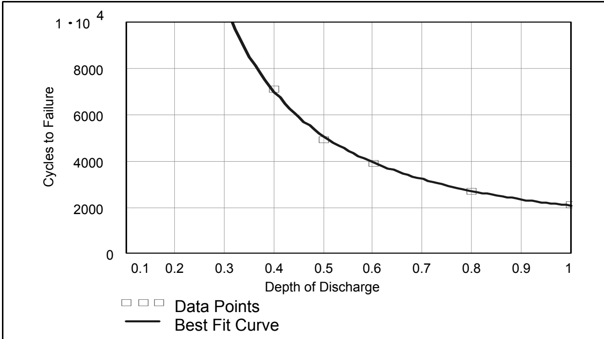
Figure 1 Best fit curve to manufacturer's cycle life data for pocket plate NiCd cells. Equation 3 parameters are u_0 = 1.67 , u_1 = -0.52 , and u_2 = 2055 .
