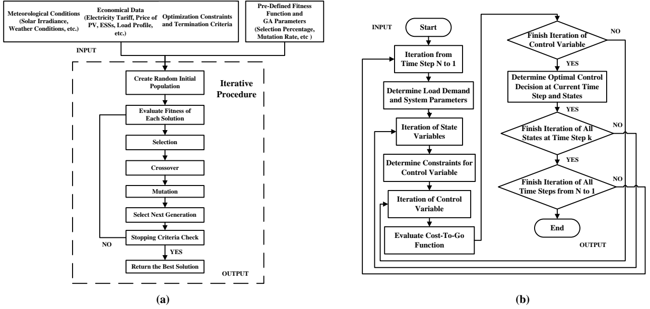
Fig. 9. Algorithm Examples of Global Optimization Approach
