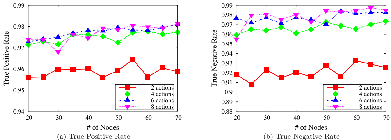
Figure 9: True Positive and Negative Rates versus # of Accumulated Actions and # of Nodes
