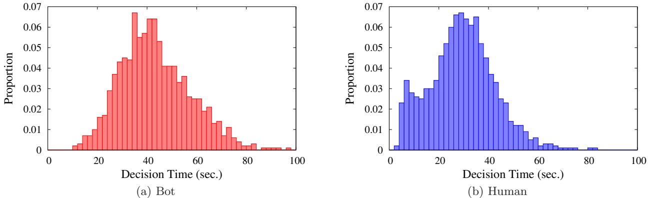
Figure 10: Decision Time Distribution
