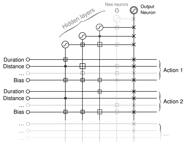
Figure 8: A Cascade Neural Network
