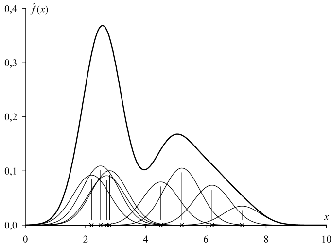
Fig. 2. Kernel estimator with smoothing parameter modification.
