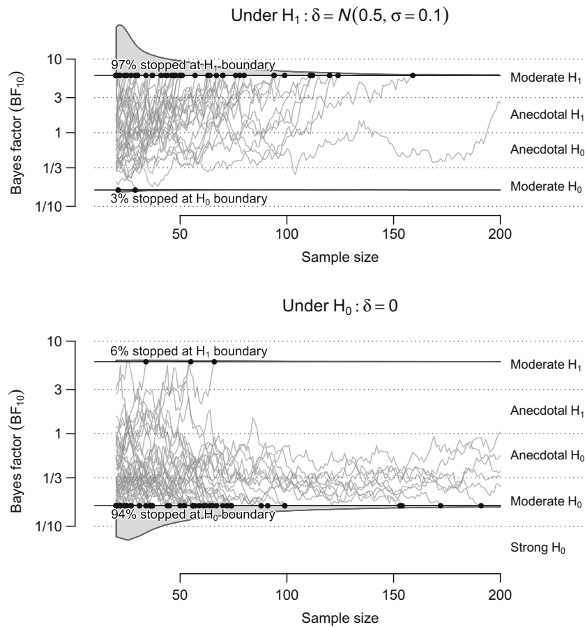
Fig. 4 The open-ended Sequential Bayes Factor design. The density of sample sizes at the stopping point and the example trajectories are based on a true effect size of \delta \sim \mathcal{N}(0.5, \sigma = 0.1) under \mathcal{H}_1 and evidential thresholds at 6 and 1/6. Figure available at https://osf.io/qny5x , under a CC-BY4.0 license
