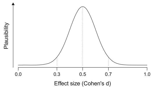
Fig. 1 A hypothetical prior distribution expressing the uncertainty about the true effect size. Figure available at https://osf.io/qny5x/ , under a CC-BY4.0 license
