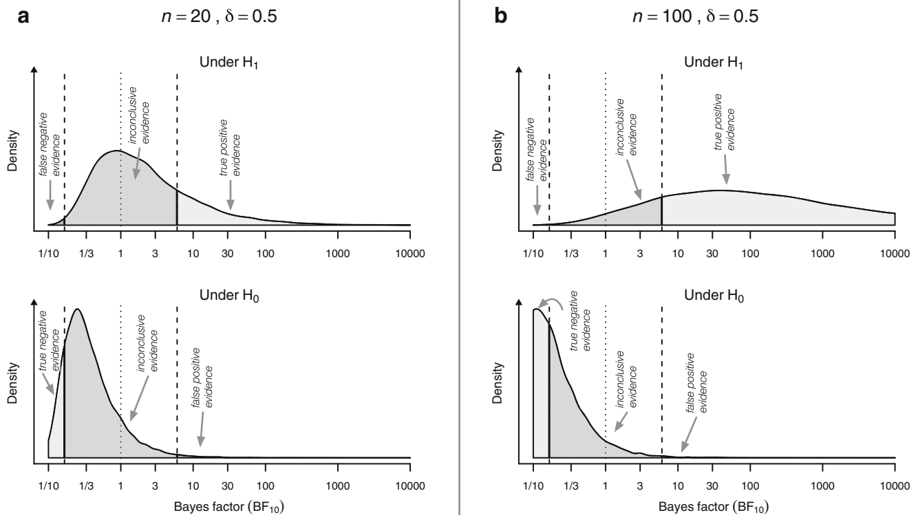
Fig. 3 Distributions of BF_{10} for a fixed- n design with a true effect size of \delta = 0.5 under \mathcal{H}_1 and a fixed n of 20 (left column), resp. 100 (right column). Distributions were categorized at BF thresholds of 1/6 and 6 . Figure available at https://osf.io/qny5x , under a CC-BY4.0 license
