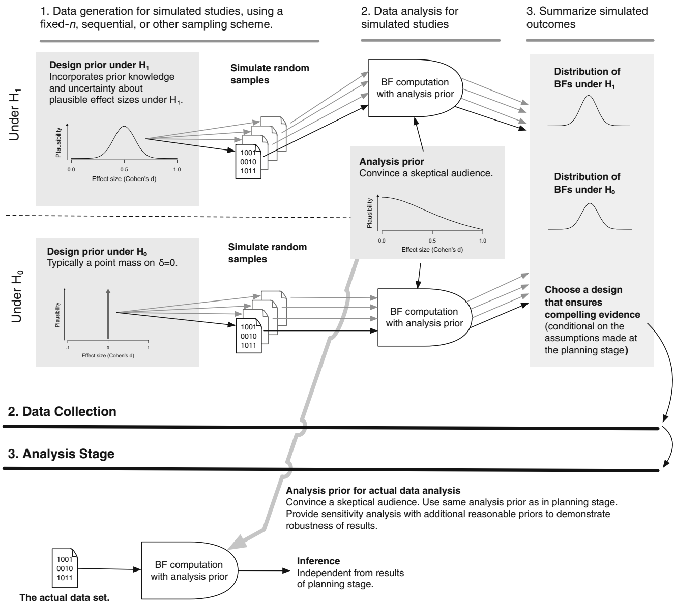
Fig. 2 Overview of the planning and analysis stages in a Monte Carlo Bayes factor design analysis. Figure available at https://osf.io/qny5x , under a CC-BY4.0 license
