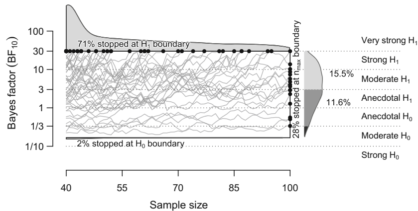
Fig. 5 The Sequential Bayes Factor With Maximal n design under \mathcal{H}_1 (results under \mathcal{H}_0 not shown). The densities and example trajectories are based on a true effect size of \delta \sim \mathcal{N}(0.5, \sigma = 0.1) , evidential thresholds at 30 and 1/6 , and n_{\max} = 100 in each group. Figure available at https://osf.io/qny5x , under a CC-BY4.0 license
