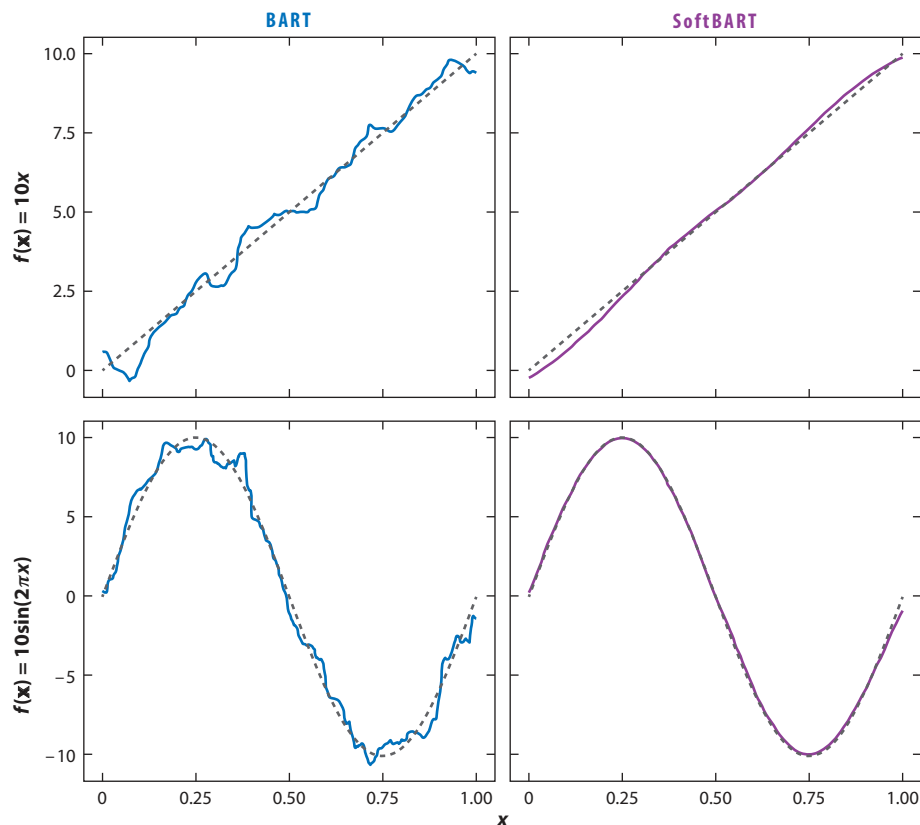
Figure 3 Posterior means (solid lines) against underlying true regression function (dashed lines). The left panels display the estimate of f(\mathbf{x}) when BART is used to estimate (top) f(\mathbf{x}) = 10x and (bottom) f(\mathbf{x}) = 10 \sin(2\pi x) . Error variance is \sigma^2 = 2^2 . The right panels show estimates using a soft version of BART. Adapted with permission from Linero & Yang (2018).
