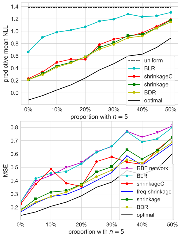
Figure 4: Top: negative log-likelihood. Bottom: mean-squared error. For context, performance of the Bayes-optimal predictor is also shown, and for NLL ‘uniform’ shows the performance of a uniform prediction on the possible labels. For MSE, the constant overall mean label predictor achieves about 1.3.
