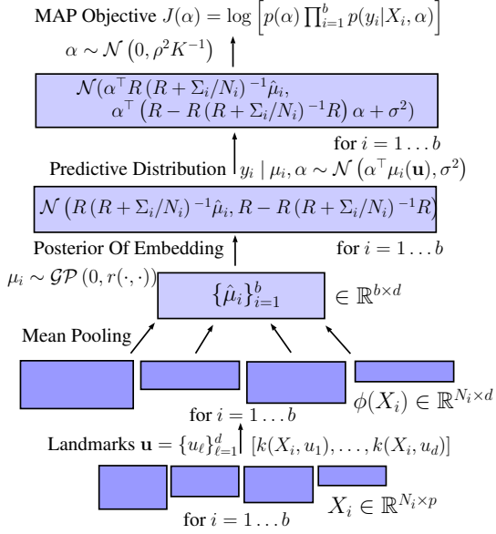
Figure 3: Our Bayesian mean shrinkage pooling model. This diagram takes m_0 = \mathbf{0} , \eta = 1 and \mathbf{u} = \mathbf{z} , so that R = R_{\mathbf{z}} = R_{\mathbf{z}\mathbf{z}} , and K_{\mathbf{z}} = K .
