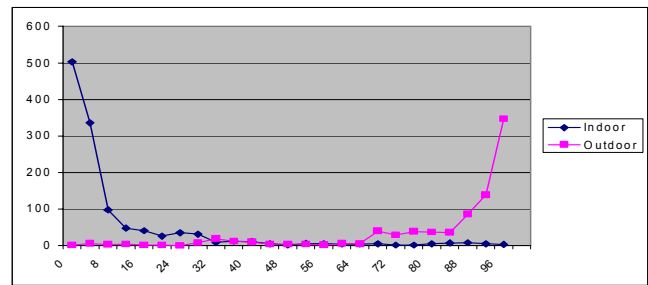
Figure 8. Distributions of beliefs for indoor and outdoor scenes shows that belief is a good measure of confidence.
