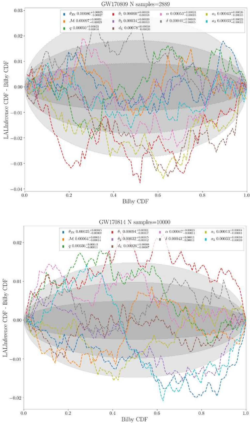
Figure D4. CDF comparison between BILBY and LALINFERENCE for GW170809 and GW170814.
