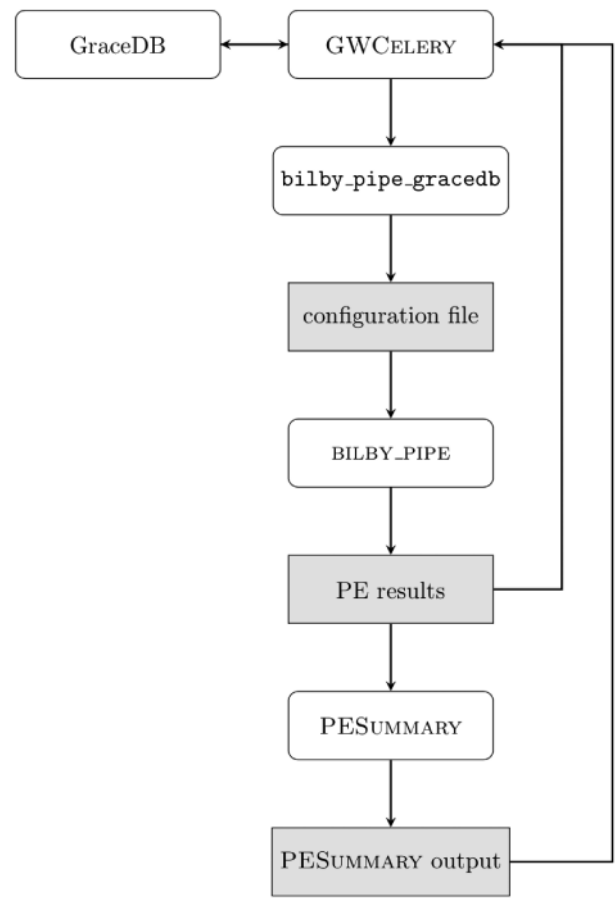
Figure 5. Workflow for online BILBY parameter estimation.
