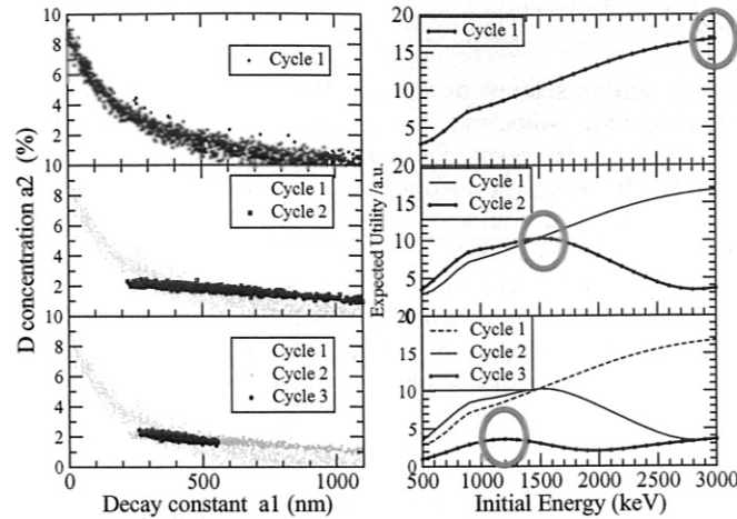
FIG. 51 Three cycles of the experimental design process; On the left hand side 1000 samples drawn from the posterior distribution p(a_1, a_2 | d, \eta) are displayed. On the right hand side the expected utility is plotted and the maximum is indicated by a circle. The corresponding abscissa value is the suggested next measurement energy. Performing that measurement yields the posterior samples (black dots) given in the second row, left hand side. The previous posterior samples are given in grey for comparison. On the right hand side the new expected utility as function of beam energy is given. Adding a new measurement with the proposed energy results in the posterior sample displayed in the lower left panel. The previous posterior samples are also given in different colors. The posterior volume has already decreased significantly. Therefore the best EU for the next measurement is lower than before (adapted from (von Toussaint et al. , 2008)).
