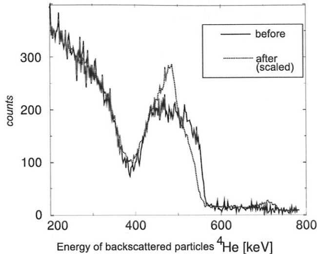
FIG. 10 RBS data of the sample before and after plasma exposition. The signal edge position at around 550 keV is shifted towards lower energies due to the plasma exposition. At the same time the peak intensity increases relative to the bulk signal. (adapted from (von Toussaint and Dose, 2006))
