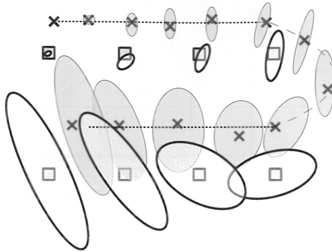
FIG. 44 The Extended Kalman Filter (EKF) applied to the robot mapping problem. The robot's path is indicated by the dotted line, and its estimations of its own position are shown as (blue) shaded ellipses which may deviate from the true position (indicated by crosses). Eight distinguishable landmarks of unknown location are indicated by small squares, and their location estimates by the robot are shown as open ellipses. During the path the robot's positional uncertainty is increasing, as is its uncertainty about the landmarks it encounters (based on Russell and Norvig (2003)).
