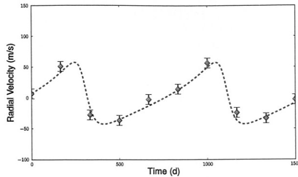
FIG. 46 The true velocity curve used for the generation of mock data is displayed as dashed line, From this velocity curve ten simulated observations distorted with Gaussian noise have been generated. These observations are given as points with error bars (from (Loredo and Chernoff, 2003b)).
