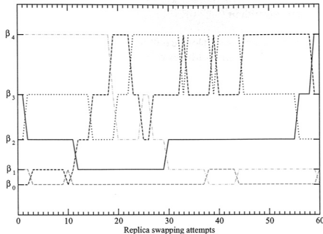
FIG. 19 Example of a typical parallel tempering run with 5 replicas at different temperatures 0 = \beta_0 < \beta_1 < \dots < \beta_4 = 1 . The average time of the replicas to swap from \beta = 0 to \beta = 1 and back is a measure of the efficiency of a parallel tempering scheme.
