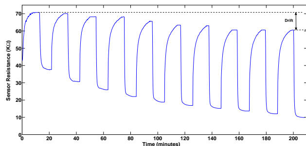
Figure 2. Typical sensor response to formaldehyde at ten different concentrations.
