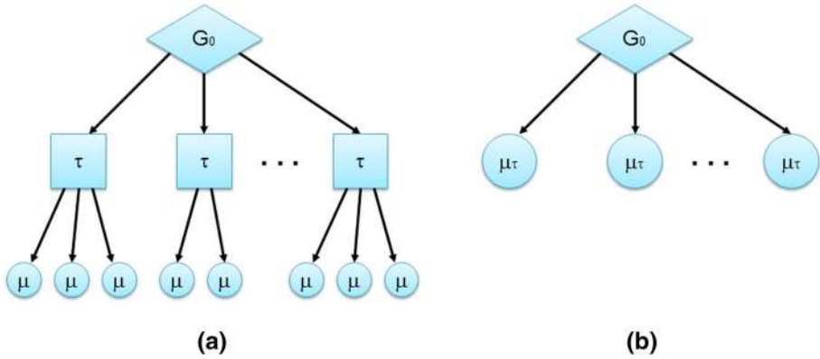
Fig. 2 Problem space abstraction model under disjoint types. a Tasks \mu are related by types \tau , with a generating distribution G_0 over them. b A simplification of the hierarchical structure under \epsilon -equivalence. The tasks of each type are represented by a single task \mu\tau
