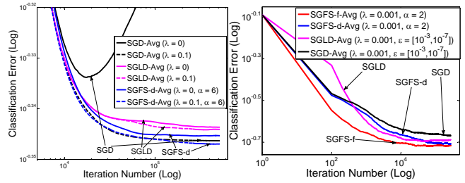
Figure 3. Test-set classification error of NNs trained with SGFS-f, SGFS-d, SGLD and SGD on the HHP dataset (left) and the MNIST dataset (right)
