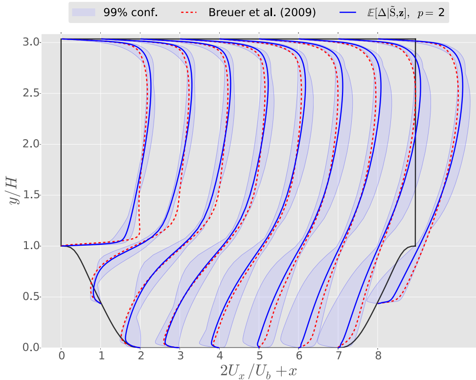
Fig. 5 BMSA for the periodic hill flow.
