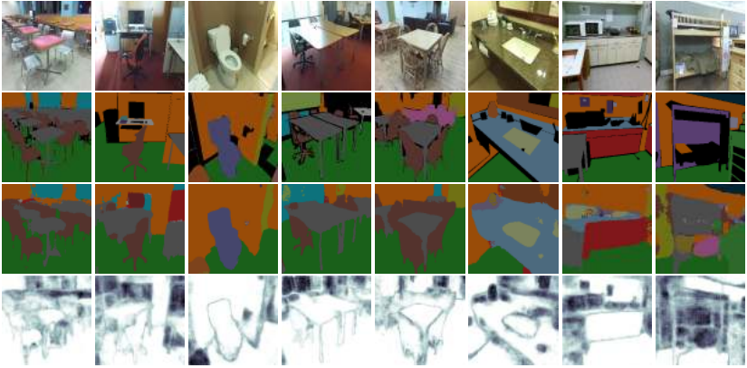
Figure 4: Bayesian SegNet results on the SUN RGB-D dataset [28] . Bayesian SegNet uses only RGB input and is able to accurately segment 37 classes in this challenging dataset.
