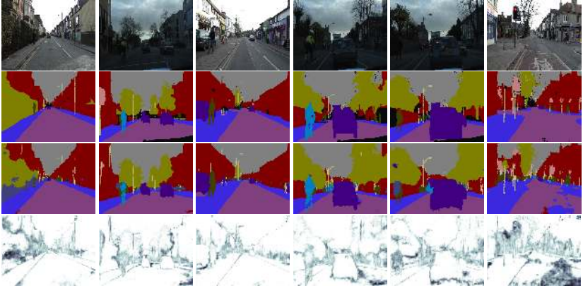
Figure 3: Bayesian SegNet results on CamVid dataset [3] . From top: input image, ground truth, Bayesian SegNet’s segmentation prediction, and overall model uncertainty averaged across all classes (with darker colours indicating more uncertain predictions).
