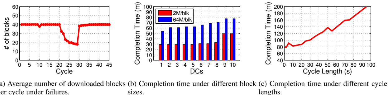
Fig. 12: BDS+'s (a) fault tolerance, (b) sensitivity to different block sizes, and (c) different cycle lengths.
