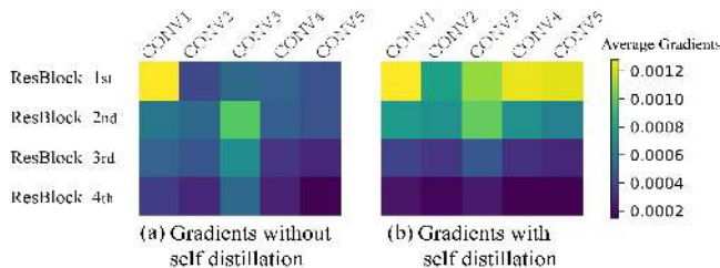
Figure 5. Statistics of layer-wised gradients.
