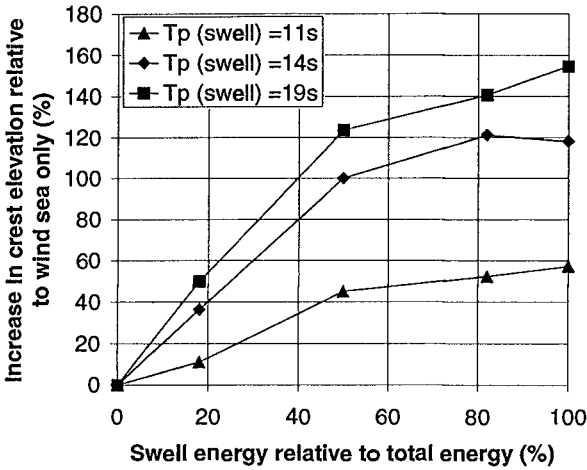
Figure 6 Relative shingle beach crest elevations under bi-modal sea conditions
