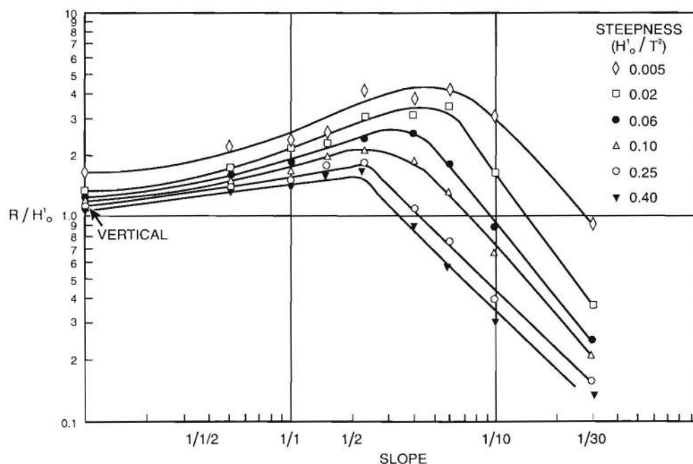
Figure 9. The relationship between relative wave run-up ( R/H_0 ), beach slope, and deep water wave steepness and height (modified from SAVAGE, 1959).
