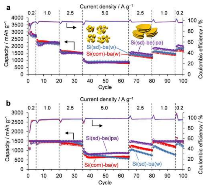
Figure 3. Charge/discharge capacities (open/solid symbols) and coulombic efficiency (solid lines) vs. cycle number. (a) Without and (b) with discharge-capacity restriction up to 1500 mAh g -1 measured in 1 M LiPF 6 in a mixture of ethylene carbonate and diethyl carbonate (1:1 by volume).
