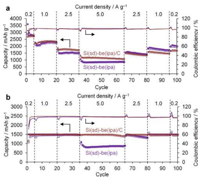
Figure 7. Charge/discharge capacities (open/solid symbols) and coulombic efficiency (solid lines) vs. cycle number (a) without and (b) with discharge-capacity restriction up to 1500 \text{ mAh g}^{-1} measured in 1 \text{ M LiPF}_6 in a mixture of ethylene carbonate and diethyl carbonate (1:1 by volume).
