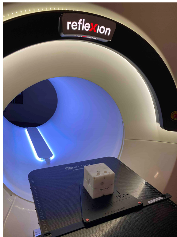
FIGURE 2 Imaging ball cube phantom setup at the external laser center
