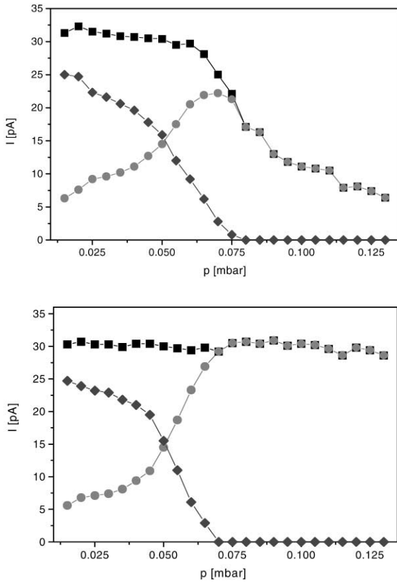
Fig. 3. The ion beam current going through the quadrupole as a function of the buffer gas pressure. The current was measured from the end plate that had a 4 mm hole in the center ( \blacklozenge ) and from a Faraday cup behind the end plate ( \bullet ). The total current reaching the end of the quadrupole is then the sum of the mentioned currents ( \blacksquare ). Top: The third deceleration electrode is at the same potential with the quadrupole. When buffer gas pressure is increased, the ions begin to leave the quadrupole from the injection side and the total current decreases. The current going through the end plate reaches zero as all the ions reaching the end of the structure are cooled and their oscillation amplitude is smaller than the end plate aperture radius. Bottom: The third deceleration electrode is at +9.5 V above the quadrupole level creating a potential barrier at the entrance. The total current remains at constant value as the number of ions going through the end plate increases with increasing buffer gas pressure. At certain pressure all the ions are cooled to an oscillation amplitude smaller than the end plate aperture radius.
