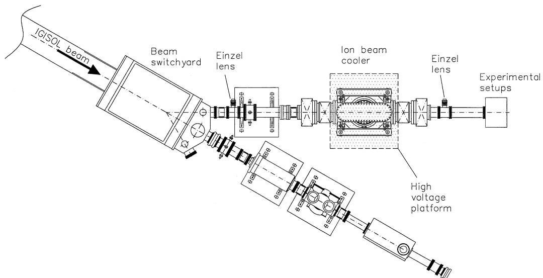
Fig. 1. IGISOL beam lines. The left beam line is reserved for the ion beam cooler and the Penning trap which is currently under construction and not shown in this figure.
