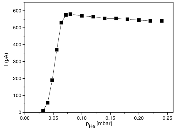
Fig. 4. Ion current transmitted through the cooler as a function of buffer gas pressure measured from a ^{89}Y^+ beam extracted and accelerated to 40 keV. The curve shows that below a certain critical pressure ions suffer no collisions and thus their oscillation is not damped. Consequently, the characteristic oscillation amplitude is far too big for any ion to survive through the miniature quadrupole. As the pressure is increased, the number of ions that are radially cooled enough that they are captured and transported out of the cooler by the miniature quadrupole, is also increased. After the maximum is reached, increase of buffer gas pressure leads to no significant loss of ions.
