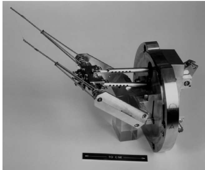
Fig. 18 Fast wire-scanner. The wire, extended between the tips of the lightweight arms, actually is a twisted strand of 15 C wires, each 6 \mu\text{m} in diameter and thus barely visible.
