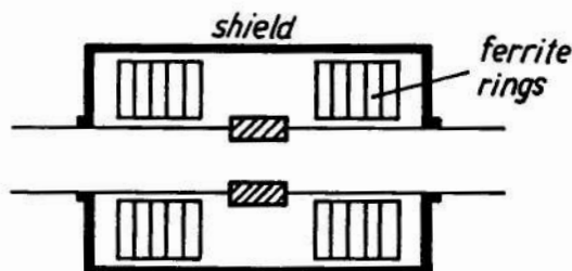
Fig. 9 Gap of WCM with shield and ferrite loading.
