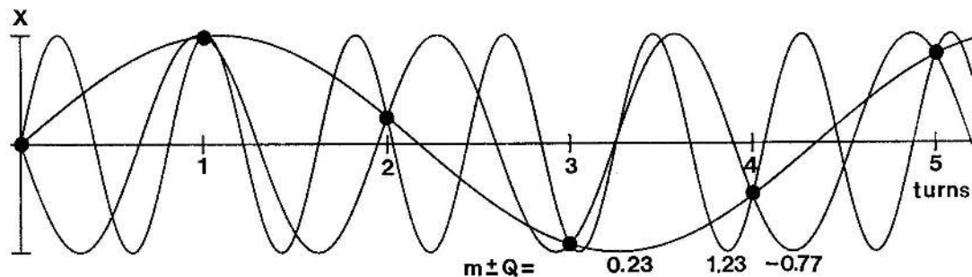
Fig. 32 Beam position on six subsequent turns and the three lowest-frequency fits.
