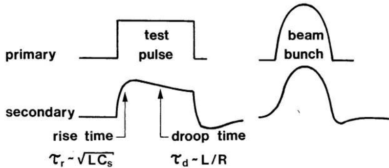
Fig. 4 Signal from real BT.
