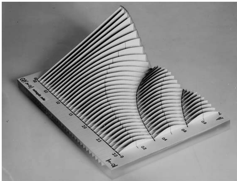
Fig. 34 Response function (vertical axis) for a rectangular kick, as a function of f_m/f_{rev} (left axis) and t_{kick}/t_{rev} (right axis).
