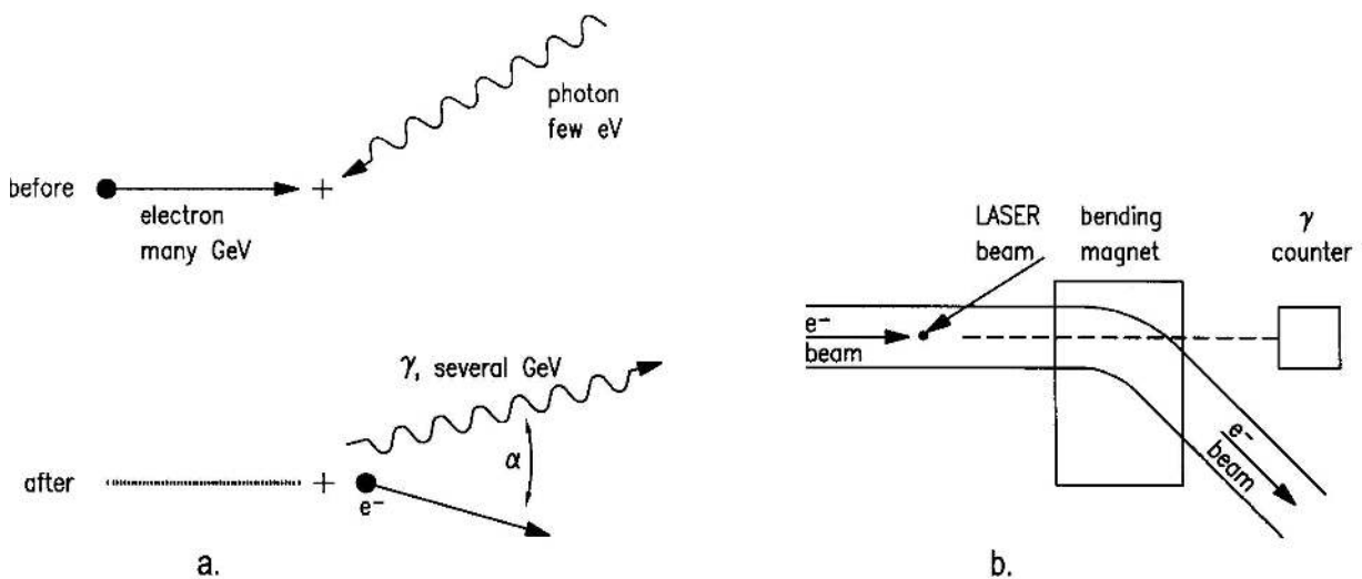
Fig. 28 a) The mechanism of Compton scattering. b) Shining LASER light on an electron beam produces high energy photons, which fly straight on at the next bending magnet.
