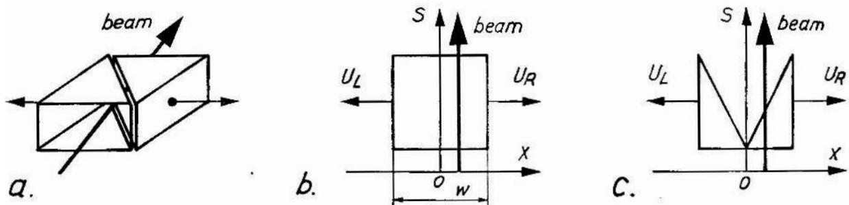
Fig. 10 a) Diagonally cut "shoe-box" PU. b) Basic geometry and tapping of signals. c) A variant which allows interleaving of a horizontal and a vertical PU.
