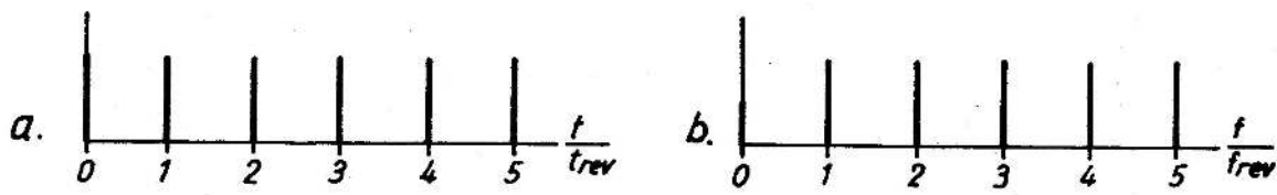
Fig. 35 a) Time domain : signal on a PU from a single circulating particle b) Frequency domain : corresponding spectrum.
