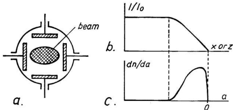
Fig. 29 a) Scraper with four blades for horizontal and vertical measurement. b) Beam intensity vs. blade position. c) Amplitude distribution.
