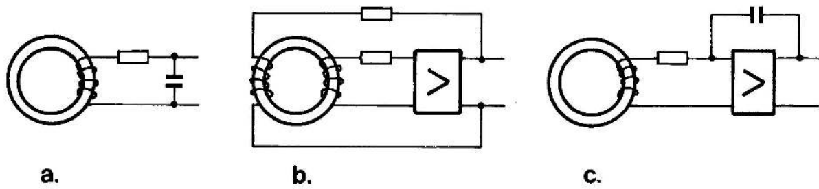
Fig. 6 Integration of signal from a BT.
