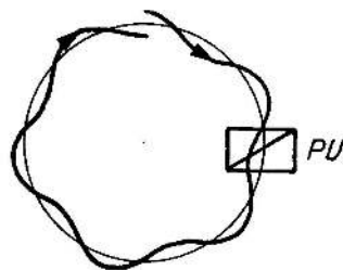
Fig. 31 A single PU records the position of an oscillating beam at every revolution.
