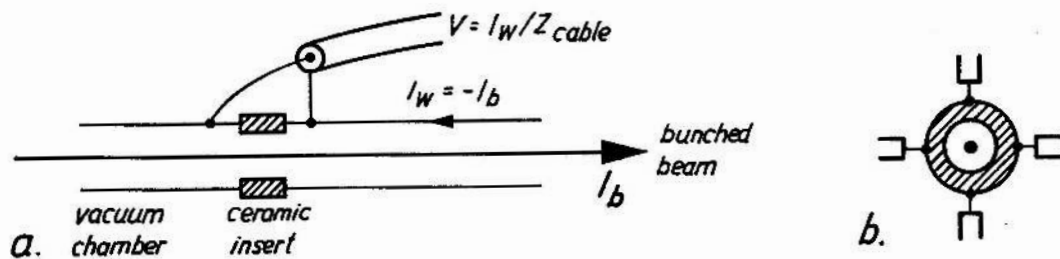
Fig. 8 a) Principle of a WCM. b) Separate pick-up of signals to observe beam position.
