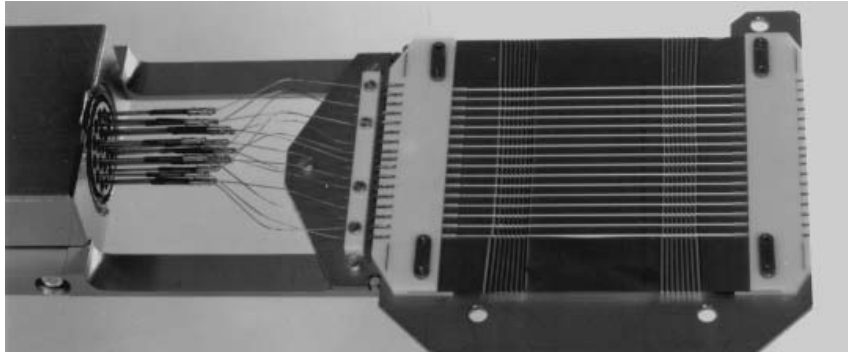
Fig. 17 A SEM made of thin ribbons attached to contacts on a ceramic frame.
