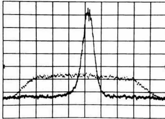
Fig. 37 Schottky scans before and after momentum cooling of 6 \times 10^6 \bar{p} in the Antiproton Accumulator. The scan is made around h = 170 , at 314 MHz.
