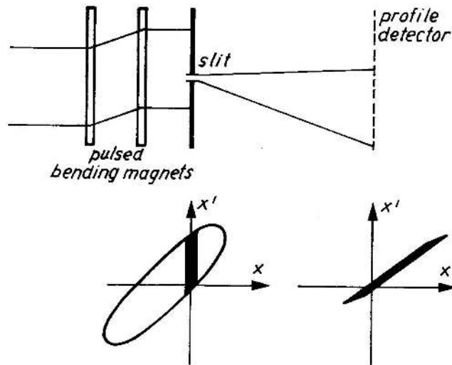
Fig. 40 Phase-space scanning to measure emittance. Above, the basic concept; underneath, the phase-space situation at the slit and at the profile detector.
