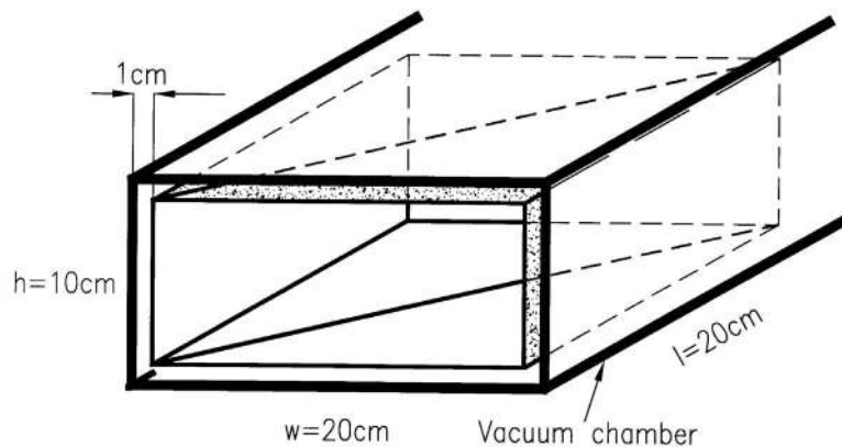
Fig. 42 Rectangular shoe-box PU inside a rectangular vacuum chamber. The dimensions are those of the electrodes.
