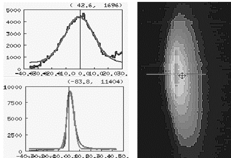
Fig. 26 Slow-extracted beam from the CERN PS. The TV image of a scintillator screen has been data-treated to yield the horizontal and vertical density profiles (left side), and a brightness-coded beam cross-section (right side).
