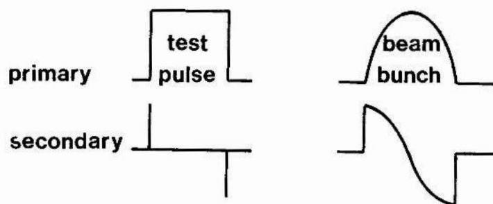
Fig. 2 Signal from an idealised BT into an infinite impedance.
