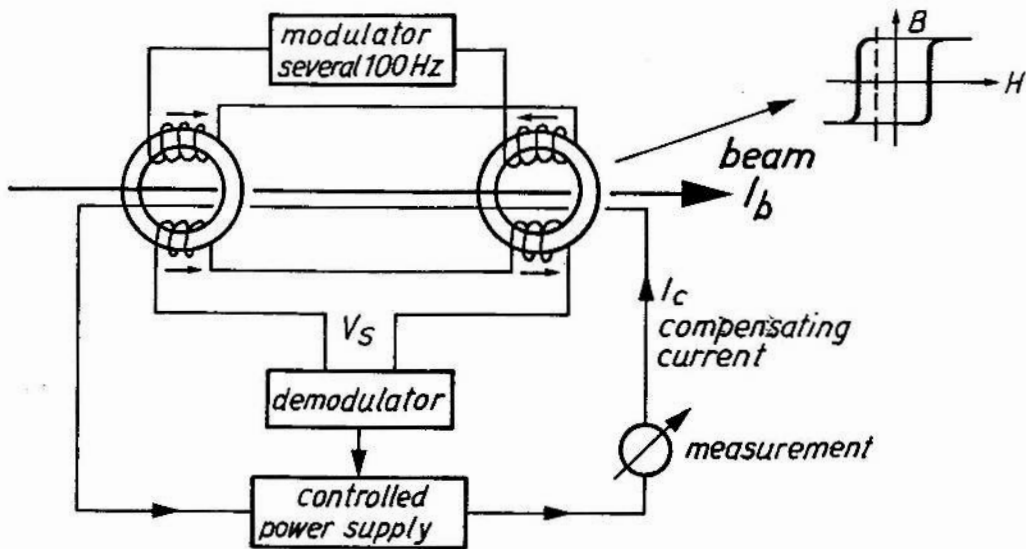
Fig. 7 Basic scheme of a dc-BT and rectangular hysteresis of core material.
