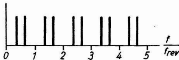
Fig. 38 The signal from a position-sensitive PU contains the frequencies f_m of the "betatron sidebands". Here, the non-integer part of Q is 0.35 or 0.65.
