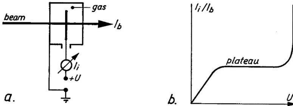
Fig. 20 a) Ionization chamber. b) Collection efficiency vs. voltage.
