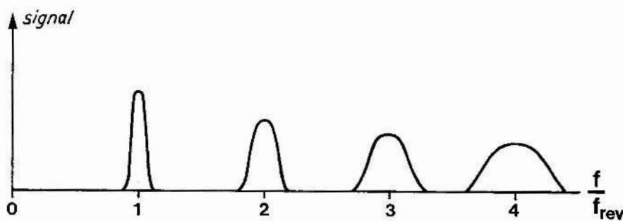
Fig. 36 Schottky scan of a many-particle beam with a spread in momentum and therefore in frequency.
