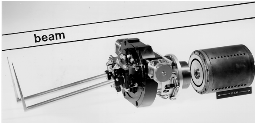
Fig. 30 Fast flip-target. The position of the blades is preadjusted outside the beam.
