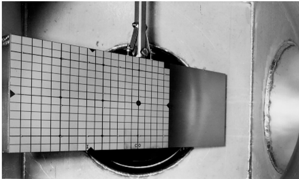
Fig. 24 Scintillator screen made from a Cr-doped Al 2 O 3 plate with imprinted graticule.
