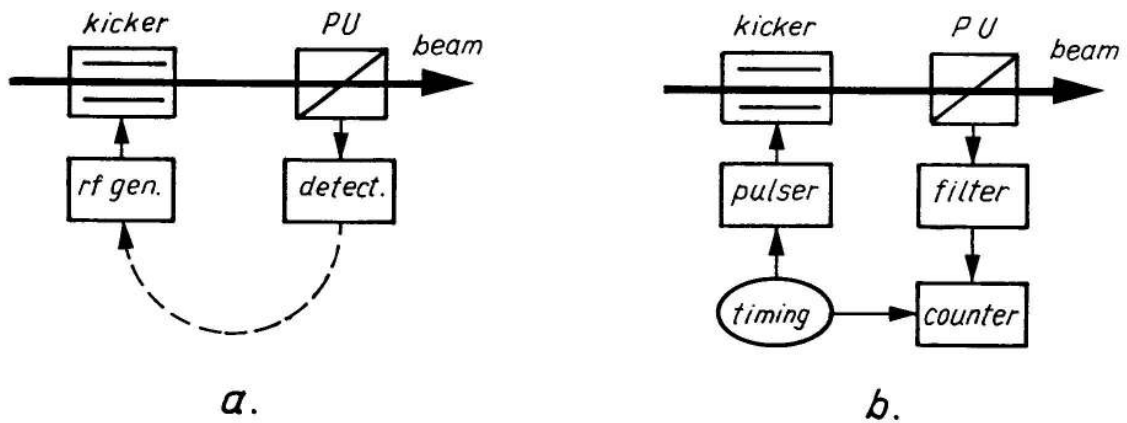
Fig. 33 Q-measurement. a) RF excitation; a feedback loop may provide lock-on. b) Application of a single short kick.
