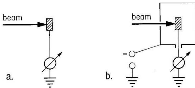
Fig. 15 a) Simple collector; b) Proper Faraday Cup.
