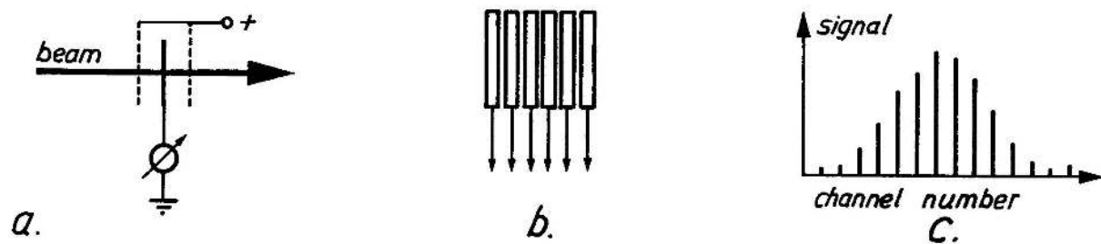
Fig. 16 a) Basic SEM: foil with clearing electrodes, seen sideways. b) A SEM consisting of an array of ribbons, seen in beam direction. c) Transverse beam profile obtained from an array of ribbons or wires.
