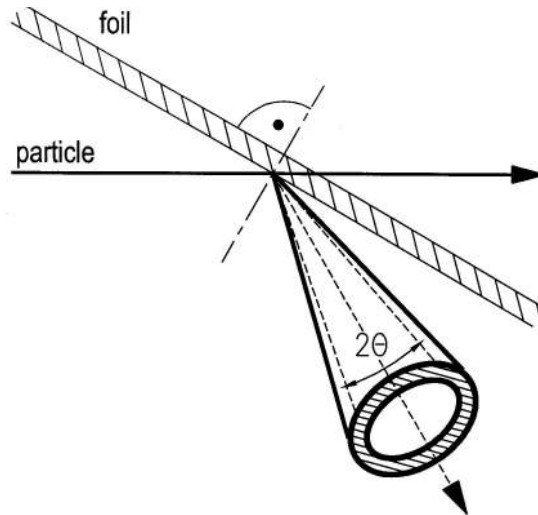
Fig. 27 OTR emitted from the entrance side of a foil. The radiation occurs into a hollow cone of opening-angle 2\theta around the "specular angle" (at which the particle would be reflected if it were a ray of light, and the foil a mirror). \theta = 1/\gamma of the particle.
