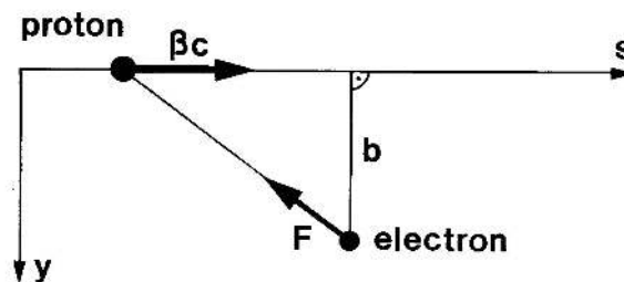
Fig. 43 Encounter between a beam particle and a shell electron. F : Coulomb force, b : impact parameter.
