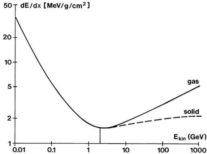
Fig. 44. Typical energy loss of a proton in matter, as a function of kinetic energy.
