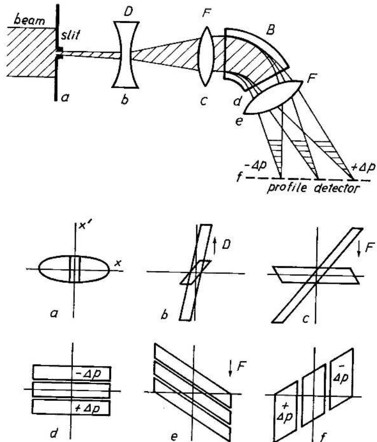
Fig. 41 Above: Basic layout of a spectrometer. D : defocusing lens, F : focusing lens, B : bending magnet. Underneath : the situation in phase space at the six significant locations a - f.
