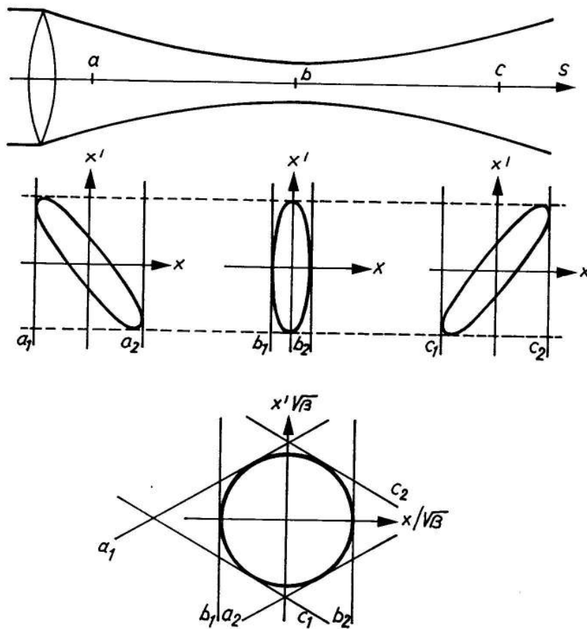
Fig. 39 Emittance ellipses at three locations: at a waist and 60^\circ in betatron phase to either side. Transforming the size-defining lines a_1, a_2, c_1, c_2 to location b , defines the emittance there.
