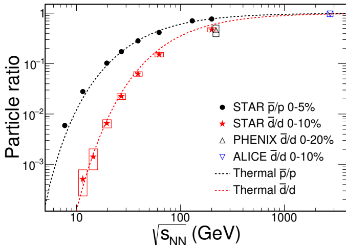
FIG. 9. Energy dependence of \bar{p}/p , \bar{d}/d ratios from Au+Au collisions at RHIC [44]. The PHENIX and ALICE data points are shown as triangles and inverted triangles [13, 33]. The curves are thermal model results as described in the text.
