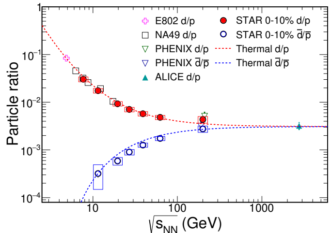
FIG. 10. Energy dependence of d/p and \bar{d}/\bar{p} yield ratios. The curves represent the thermal model results as described in the text. The symbols represent measured data [13, 29, 33, 36].
