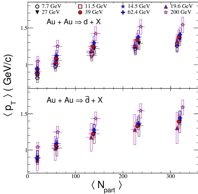
FIG. 7. Centrality dependence of \langle p_T \rangle of deuterons (top panel) and anti-deuterons (bottom panel) in Au+Au collisions at \sqrt{s_{NN}} = 7.7, 11.5, 14.5, 19.6, 27, 39, 62.4, and 200 GeV. The \bar{d} results at 11.5 and 14.5 GeV are not presented due to their large uncertainty. The statistical and systematical uncertainties are shown as vertical lines and boxes, respectively.
