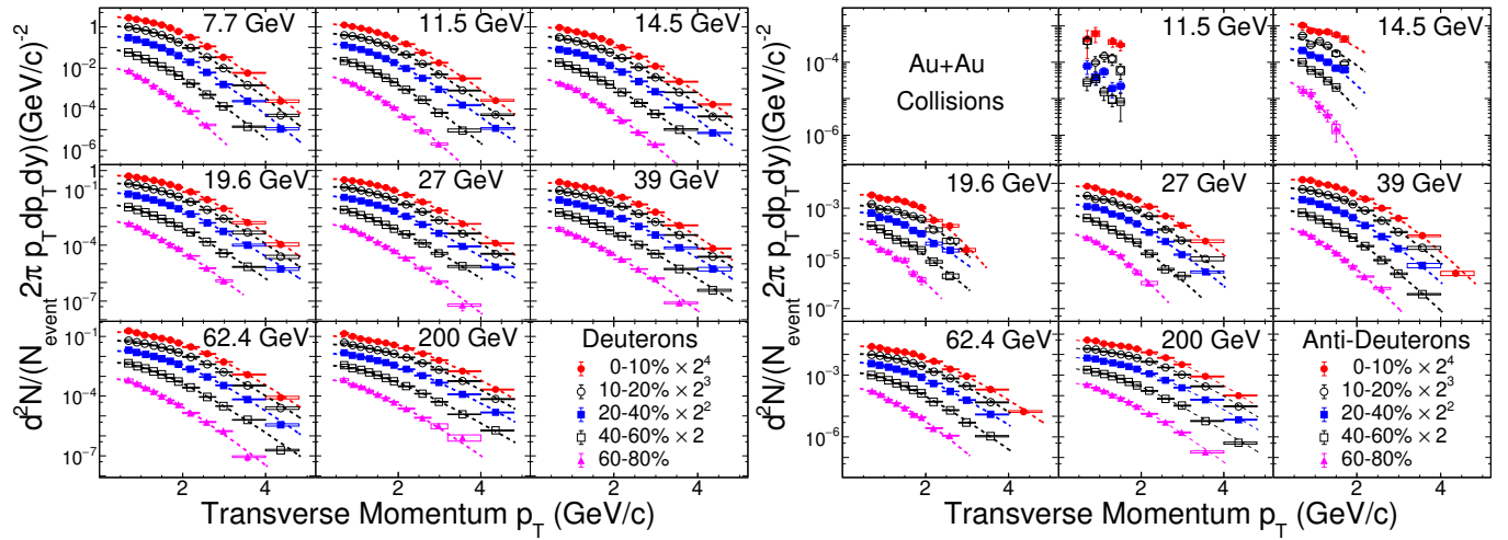
FIG. 6. Mid-rapidity ( |y| < 0.3 ) transverse momentum spectra for deuterons and anti-deuterons in Au+Au collisions at \sqrt{s_{NN}} = 7.7, 11.5, 14.5, 19.6, 27, 39, 62.4, and 200 GeV for 0–10%, 10–20%, 20–40%, 40–60%, and 60–80% centralities. There are not enough candidates to obtain the anti-deuterons p_T spectra at \sqrt{s_{NN}} = 7.7 GeV. The dashed-lines are the results of the Blast-Wave fits to each distribution with the profile parameter n=1 , see discussions in the text. The statistical and systematical uncertainties are shown as vertical-lines and boxes, respectively. Horizontal uncertainties reflect the p_T bin width used in the analysis. The spectra for different centralities are scaled for clarity.
