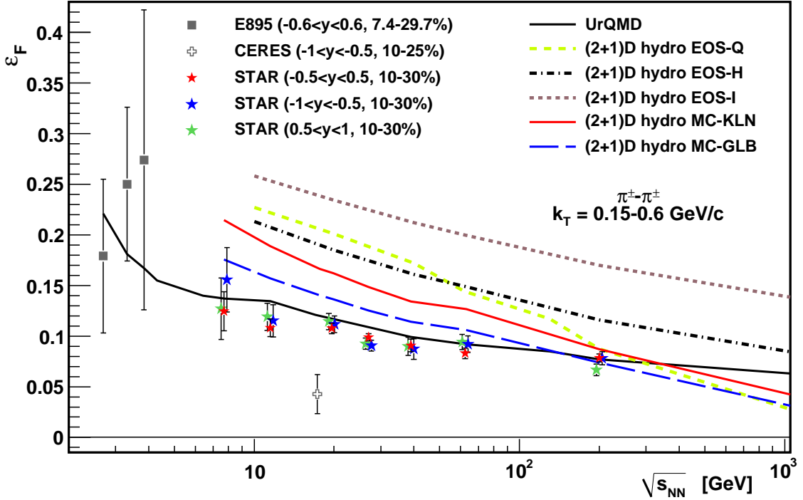
FIG. 27: (Color online) The dependence of the kinetic freeze-out eccentricity of pions on collision energy in mid-central Au+Au collisions (E895, STAR) and Pb+Au collisions (CERES) for three rapidity regions and with \langle k_T \rangle \approx 0.31 GeV/c. For clarity, the points for forward and backward rapidity from STAR are offset slightly. Error bars include only statistical uncertainties. Several (2+1)D hydrodynamical models and UrQMD calculations are shown. Model centralities correspond to the data. The trend is consistent with a monotonic decrease in eccentricity with beam energy.
