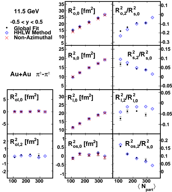
FIG. 13: (Color online) Centrality dependence of the Fourier coefficients that describe azimuthal oscillations of the HBT radii, at mid-rapidity ( -0.5 < y < 0.5 ), in 11.5 GeV collisions with \langle k_T \rangle \approx 0.31 GeV/c. The symbols have the same meaning as in Fig. 11. Error bars include only statistical uncertainties. The 0-5% global fit point is excluded.
