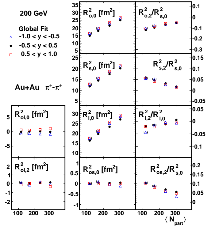
FIG. 24: (Color online) Centrality dependence of the Fourier coefficients that describe azimuthal oscillations of the HBT radii, at backward ( -1 < y < -0.5 ), forward ( 0.5 < y < 1 ) and mid ( -0.5 < y < 0.5 ) rapidity, in 200 GeV collisions with \langle k_T \rangle \approx 0.31 GeV/c using the global fit method. Error bars include only statistical uncertainties. The 0-5% global fit point is excluded.
