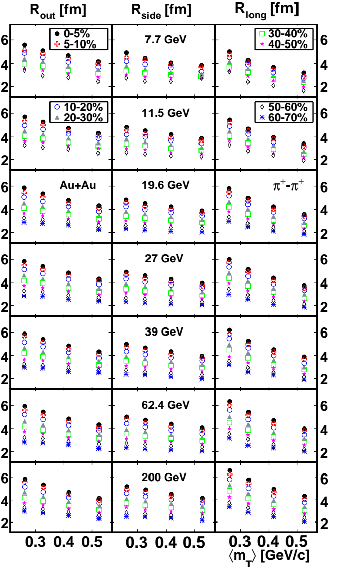
FIG. 7: (Color online) The \langle m_T \rangle dependence of R_{out} , R_{side} and R_{long} for each energy and multiple centralities. Errors are statistical only. For 7.7 GeV and 11.5 GeV, the results for 60-70% centrality are excluded due to lack of statistics.
