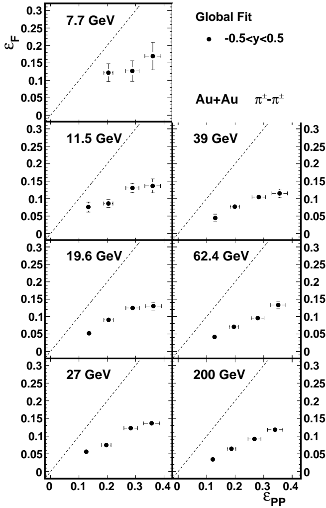
FIG. 26: The eccentricity of the collisions at kinetic freeze-out, \epsilon_F , as a function of initial eccentricity relative to the participant plane, \epsilon_{PP} , at mid-rapidity. All results are for \langle k_T \rangle \approx 0.31 GeV/c. Error bars include only statistical uncertainties. The line has a slope of one indicating no change in shape. Points further below the line evolve more to a round shape.
