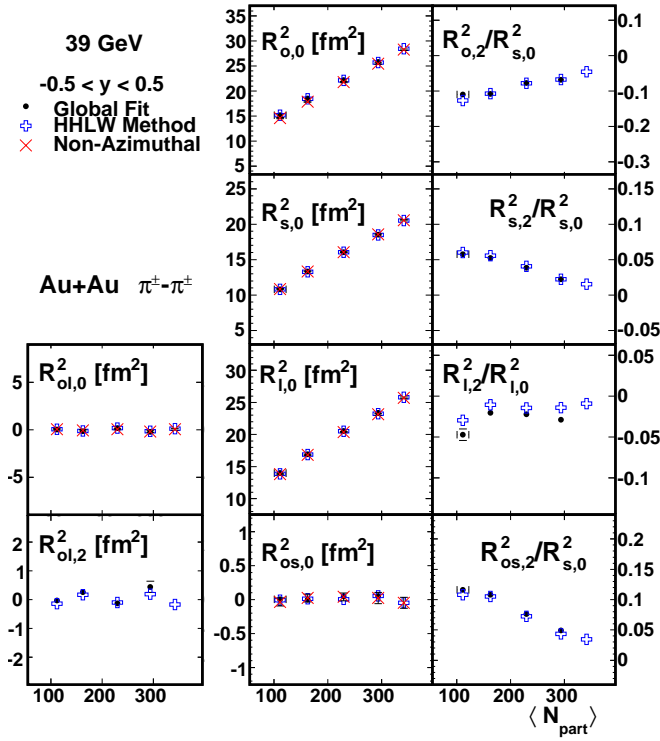
FIG. 19: (Color online) Centrality dependence of the Fourier coefficients that describe azimuthal oscillations of the HBT radii, at mid-rapidity ( -0.5 < y < 0.5 ), in 39 GeV collisions with \langle k_T \rangle \approx 0.31 GeV/c. The symbols have the same meaning as in Fig. 11. Error bars include only statistical uncertainties. The 0-5% global fit method point is excluded.
