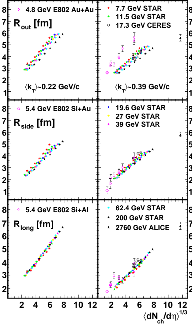
FIG. 8: (Color online) The dependence of the HBT radii on multiplicity, \langle dN_{ch}/d\eta \rangle^{1/3} , for \langle k_T \rangle \approx 0.22 GeV/c (left) and \langle k_T \rangle \approx 0.39 GeV/c (right). Results are for Au+Au collisions at STAR, Pb+Au at CERES [28], Pb+Pb at ALICE [36], and Si+A at E802 [25]. Errors are statistical only.
