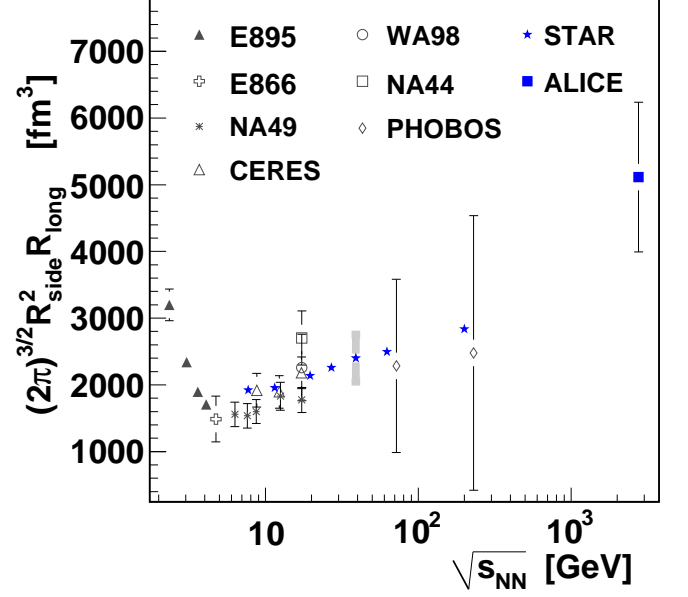
FIG. 9: (Color online) The beam energy dependence of the volume, V = (2\pi)^{3/2} R_{side}^2 R_{long} , of the regions of homogeneity at kinetic freeze-out in central Au+Au, Pb+Pb and Pb+Au collisions with \langle k_T \rangle \approx 0.22 GeV/c [26–32, 36]. The systematic errors for STAR points at all energies (from Table II) are of similar size to error bar for 39 GeV, shown as a representative example. Errors on other results are statistical only, to emphasize the trend. The PHOBOS points are offset in \sqrt{s_{NN}} for clarity. The text contains some discussion about variations in centrality, \langle k_T \rangle , and analysis techniques between different experiments.
