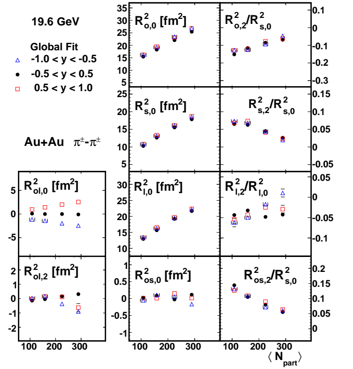
FIG. 16: (Color online) Centrality dependence of the Fourier coefficients that describe azimuthal oscillations of the HBT radii, at backward ( -1 < y < -0.5 ), forward ( 0.5 < y < 1 ) and mid ( -0.5 < y < 0.5 ) rapidity, in 19.6 GeV collisions with \langle k_T \rangle \approx 0.31 GeV/c using the global fit method. Error bars include only statistical uncertainties. The 0-5% global fit point is excluded.
