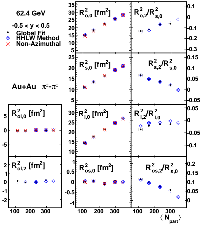
FIG. 21: (Color online) Centrality dependence of the Fourier coefficients that describe azimuthal oscillations of the HBT radii, at mid-rapidity ( -0.5 < y < 0.5 ), in 62.4 GeV collisions with \langle k_T \rangle \approx 0.31 GeV/c. The symbols have the same meaning as in Fig. 11. Error bars include only statistical uncertainties. The 0-5% global fit method point is excluded.
