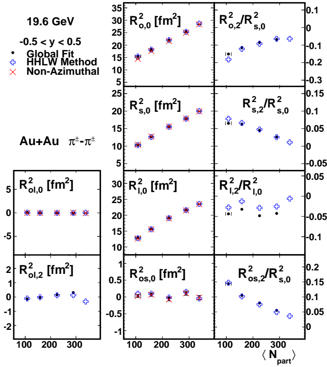
FIG. 15: (Color online) Centrality dependence of the Fourier coefficients that describe azimuthal oscillations of the HBT radii, at mid-rapidity ( -0.5 < y < 0.5 ), in 19.6 GeV collisions with \langle k_T \rangle \approx 0.31 GeV/c. The symbols have the same meaning as in Fig. 11. Error bars include only statistical uncertainties. The 0-5% global fit point is excluded.
