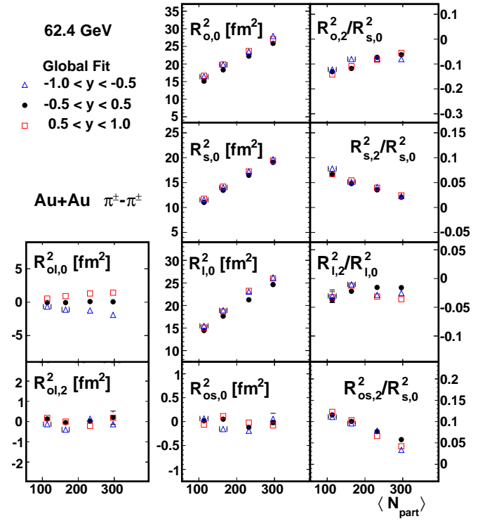
FIG. 22: (Color online) Centrality dependence of the Fourier coefficients that describe azimuthal oscillations of the HBT radii, at backward ( -1 < y < -0.5 ), forward ( 0.5 < y < 1 ) and mid ( -0.5 < y < 0.5 ) rapidity, in 62.4 GeV collisions with \langle k_T \rangle \approx 0.31 GeV/c using the global fit method. Error bars include only statistical uncertainties. The 0-5% global fit point is excluded.
