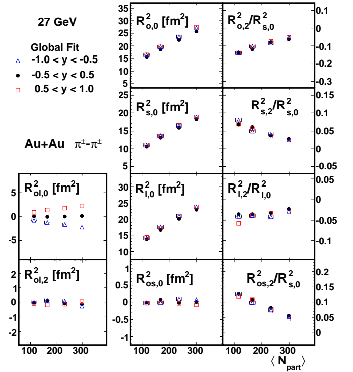
FIG. 18: (Color online) Centrality dependence of the Fourier coefficients that describe azimuthal oscillations of the HBT radii, at backward ( -1 < y < -0.5 ), forward ( 0.5 < y < 1 ) and mid ( -0.5 < y < 0.5 ) rapidity, in 27 GeV collisions with \langle k_T \rangle \approx 0.31 GeV/c using the global fit method. Error bars include only statistical uncertainties. The 0-5% global fit point is excluded.
