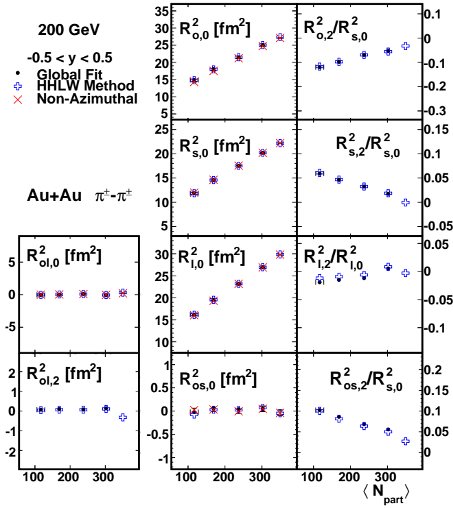
FIG. 23: (Color online) Centrality dependence of the Fourier coefficients that describe azimuthal oscillations of the HBT radii, at mid-rapidity ( -0.5 < y < 0.5 ), in 200 GeV collisions with \langle k_T \rangle \approx 0.31 GeV/c. The symbols have the same meaning as in Fig. 11. Error bars include only statistical uncertainties. The 0-5% global fit method point is excluded.
