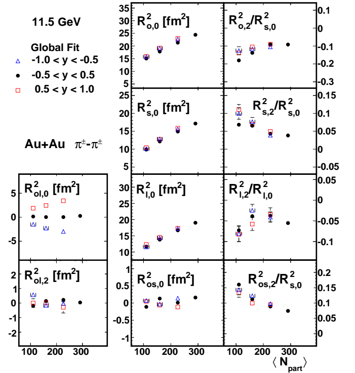
FIG. 14: (Color online) Centrality dependence of the Fourier coefficients that describe azimuthal oscillations of the HBT radii, at backward ( -1 < y < -0.5 ), forward ( 0.5 < y < 1 ) and mid ( -0.5 < y < 0.5 ) rapidity, in 11.5 GeV collisions with \langle k_T \rangle \approx 0.31 GeV/c using the global fit method. Error bars include only statistical uncertainties. The 0-5% and two 5-10% points have been excluded.
