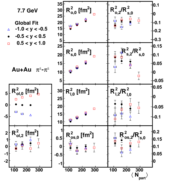
FIG. 12: (Color online) Centrality dependence of the Fourier coefficients that describe azimuthal oscillations of the HBT radii, at backward ( -1 < y < -0.5 ), forward ( 0.5 < y < 1 ) and mid ( -0.5 < y < 0.5 ) rapidity, in 7.7 GeV collisions with \langle k_T \rangle \approx 0.31 GeV/c using the global fit method. Error bars include only statistical uncertainties. The 0-5% and two 5-10% points have been excluded.
