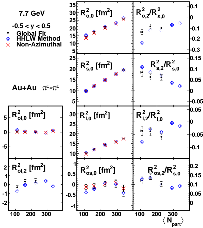
FIG. 11: (Color online) Centrality dependence of the Fourier coefficients that describe azimuthal oscillations of the HBT radii, at mid-rapidity ( -0.5 < y < 0.5 ), in 7.7 GeV collisions with \langle k_T \rangle \approx 0.31 GeV/c. Open symbols are results using separate Gaussian fits to each angular bin, the HHLW method. Solid circles represent results using a single global fit to all angular bins to directly extract the Fourier coefficients. Crosses directly compare the azimuthally integrated radii and the 0 th -order Fourier coefficients. Error bars include only statistical uncertainties. The 0-5% and 5-10% global fit points have been excluded.
