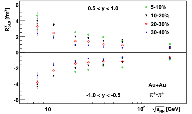
FIG. 25: (Color online) Beam energy dependence of the R_{ol,0}^2 cross term for forward and backward rapidity with \langle k_T \rangle \approx 0.31 GeV/c.
