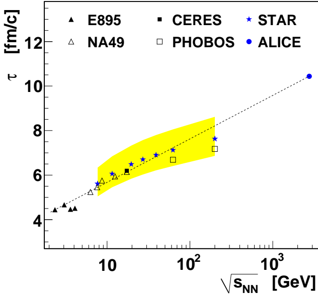
FIG. 10: (Color online) The lifetime, \tau , of the system as a function of beam energy for central Au+Au collisions assuming a temperature of T = 0.12 GeV at kinetic freeze-out. The yellow band demonstrates the effect on \tau of varying the assumed temperature by \pm 0.02 GeV. Statistical uncertainties from the fits are smaller than the data points. The line extrapolates between the lowest and highest energy. The text contains some discussion about variations in centrality and analysis techniques between different experiments.
