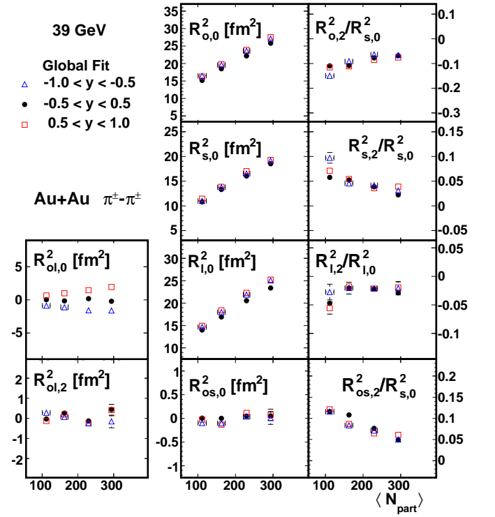
FIG. 20: (Color online) Centrality dependence of the Fourier coefficients that describe azimuthal oscillations of the HBT radii, at backward ( -1 < y < -0.5 ), forward ( 0.5 < y < 1 ) and mid ( -0.5 < y < 0.5 ) rapidity, in 39 GeV collisions with \langle k_T \rangle \approx 0.31 GeV/c using the global fit method. Error bars include only statistical uncertainties. The 0-5% global fit point is excluded.
