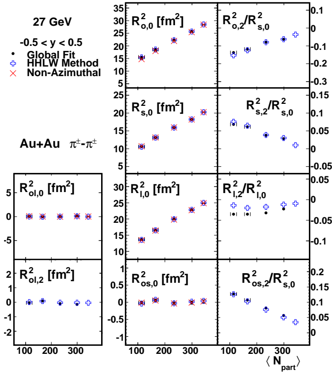
FIG. 17: (Color online) Centrality dependence of the Fourier coefficients that describe azimuthal oscillations of the HBT radii, at mid-rapidity ( -0.5 < y < 0.5 ), in 27 GeV collisions with \langle k_T \rangle \approx 0.31 GeV/c. The symbols have the same meaning as in Fig. 11. Error bars include only statistical uncertainties. The 0-5% global fit method point is excluded.
