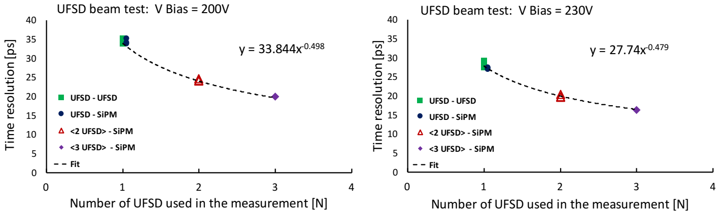
Figure 8 Timing resolution for: single UFSD (N=1) obtained from the UFSD-SiPM and UFSD-UFSD time differences; averaged pairs of UFSD (N=2) and average of 3 UFSD (N = 3) for bias voltages of (left) 200V and (right) 230V.
