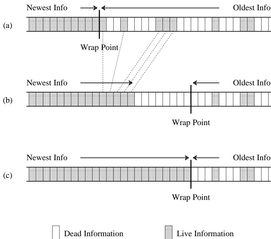
Figure 2. Incremental compaction in a log-structured file system. New data is appended to the log from left-to-right. In (a) the log has just filled up; among the oldest blocks in the log, only a few are still alive. In (b) the live information is compacted to the head of the log, leaving empty space for new log information. In (c) new information is appended to the log, regenerating the situation in (a).
