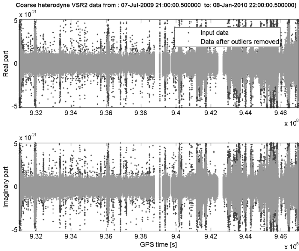
Figure 6. Coarse heterodyne data before (blue) and after (red) removal of the outliers using the Grubbs test. The top panel presents the real part of the data and the bottom panel the imaginary one. Not all the input data are shown because some outliers are large. There are 2814 and 2765 outliers outside the range of the plots for real and imaginary part of the data, respectively.
