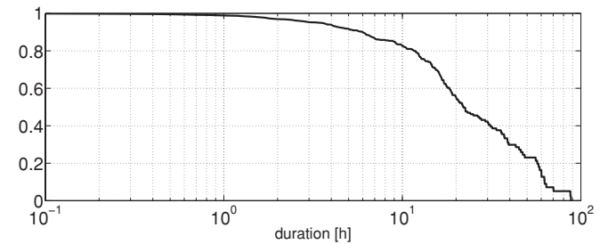
Figure 2. Fraction of the total time covered by science data segments with duration larger than a given time.
