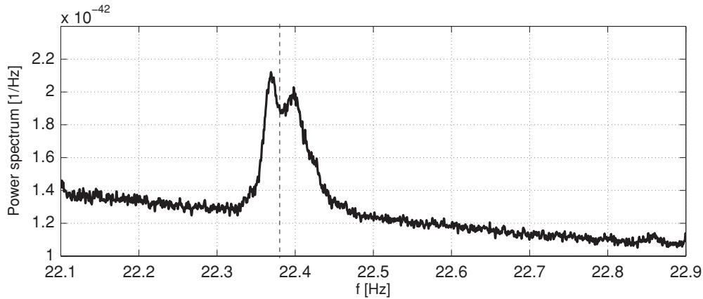
Figure 3. Estimation of the power spectrum of VSR2 data in a 0.8 Hz band around the expected Vela signal frequency. The expected signal frequency (vertical dashed line) is right in the middle of the frequency band affected by an instrumental disturbance; see the text for more details.
