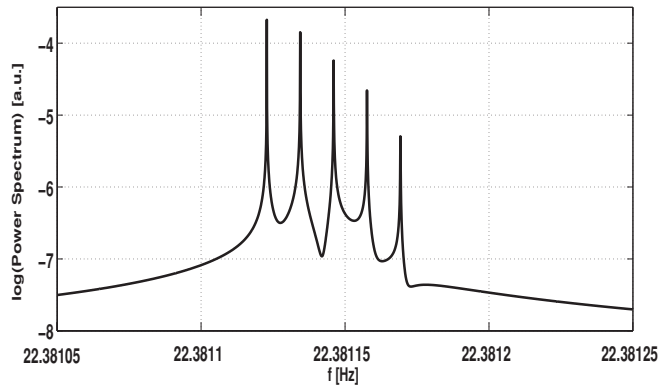
Figure 1. Power spectrum of a hypothetical monochromatic signal coming from the location of the Vela pulsar as seen from the Virgo detector. The left plot refers to a purely + signal; the right plot to a circularly (left-handed) polarized signal.
