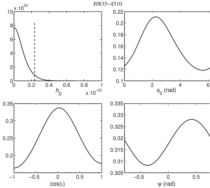
Figure 5. Posterior PDFs for the pulsar parameters h_0 , \Phi_0 , \cos i , and \psi for PSR J0835–4510, produced using uniform priors for \cos i and \psi across the range of their possible values with the complex heterodyne method. The vertical dashed line shows the 95% upper limit on h_0 .
