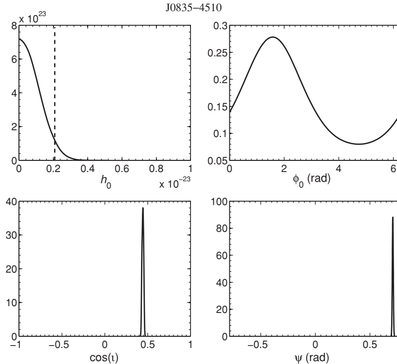
Figure 4. Posterior PDFs for the pulsar parameters h_0 , \Phi_0 , \cos i , and \psi for PSR J0835–4510, produced using restricted priors on \cos i and \psi with the complex heterodyne method. The vertical dashed line shows the 95% upper limit on h_0 .
