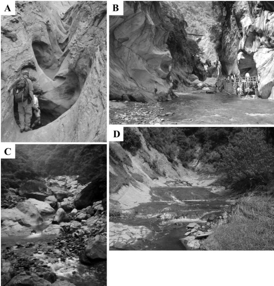
Figure 2 (A) Chain of potholes in Navajo Sandstone, Utah. (B) Gravel-bedded incised bedrock river, Taroko National Park, Taiwan. Note 1–2 m diameter flutes high on rock bank (left) indicating active suspended load abrasion. (C) Landslide-derived boulder lag, Longmenshan, China. (D) Stepped plane-bed bedrock channel in mudstone, Waipaoa catchment, North Island, New Zealand.
