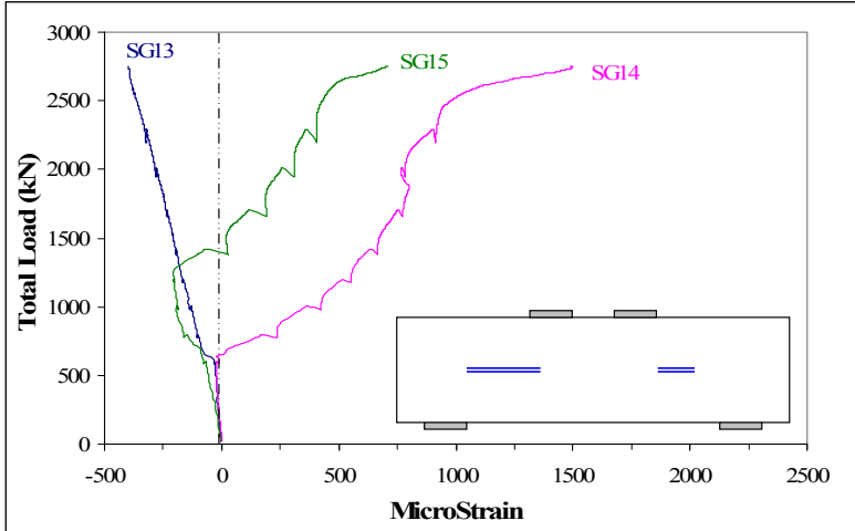
Figure A-31 Strains on the horizontal web reinforcement of specimen MS1-3
