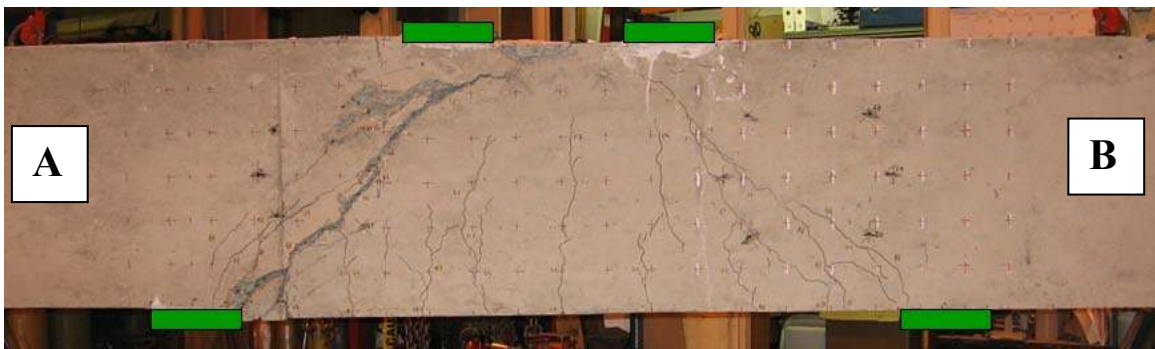
Figure 4-38 Specimen MW1-2 after failure
