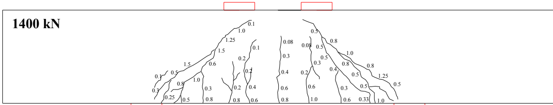
Figure A-72 Crack patterns at 1400 kN of specimen MW1-2
