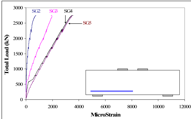
Figure A-28 Strains at a bar located in the lowest layer of main tension reinforcement of specimen MS1-3
