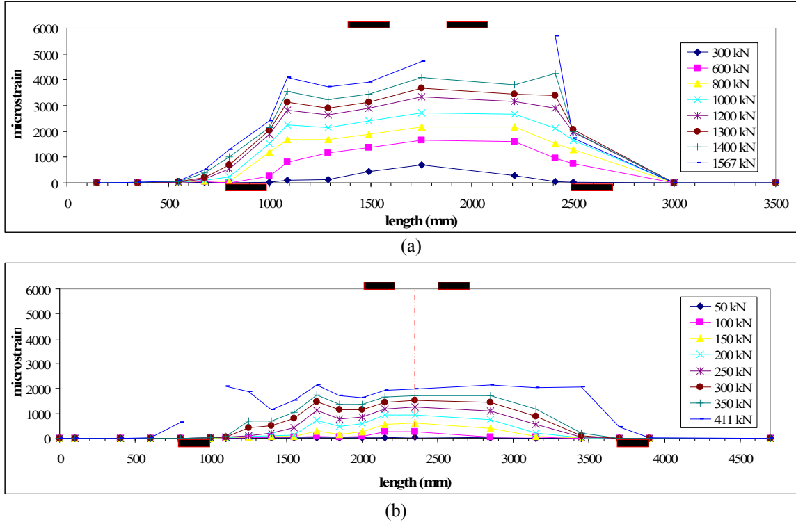
Figure 5-21 Strain distribution along the bottom bar for (a) MW1-2 and (b) MW3-2 at different loading stages
