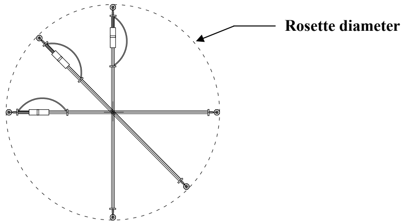
Figure 3-32 LVDT rosettes
