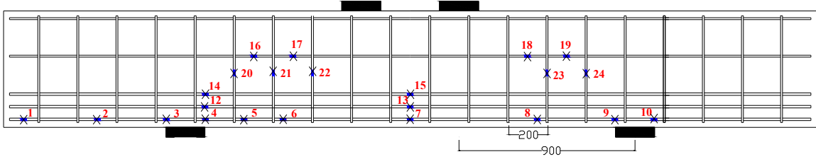
Figure A-38 Strain gauges locations of specimen MS2-2
