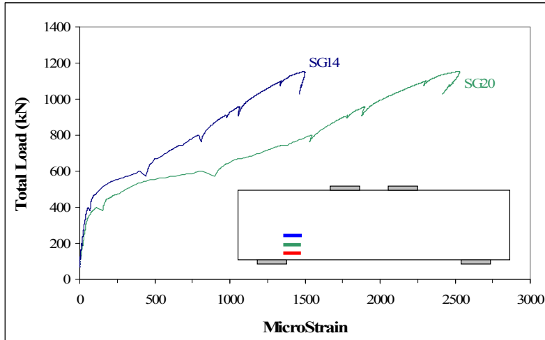
Figure A-67 Strain at the interior edge of one support for the three layers of tension reinforcement of specimen MS3-2
