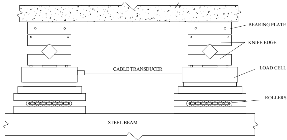
Figure 3-21 Supports details
