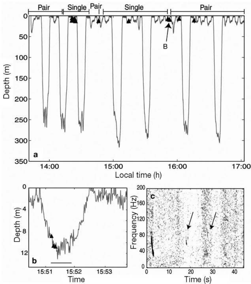
Fig. 6. Balaenoptera musculus . Dive profile for tagged whale of fluid pair observed September 28, 2003, in Monterey Bay. (a) Overall dive profile of tagged female; (▲) times of medium- and high-SNR D calls; paired status of tagged female is annotated across top axis; B: 1 calling dive, shown in greater detail in (b), in which there may be counter-calls between whales in the joining pair. (b) High- and medium-SNR calls (▲); horizontal bar indicates time period shown in (c). (c) Spectrogram showing counter-calls heard during calling dive in (b), with high-SNR call ascribed to the tagged female, and low-SNR calls (arrowed) ascribed to the untagged male in the pair
