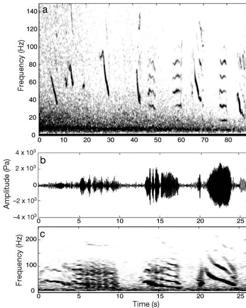
Fig. 3. Balaenoptera musculus . (a) Spectrogram of D calls and highly variable tonal calls recorded by tag on September 26, 2003, in Monterey Bay; D calls are quite variable, with different starting and ending frequencies for each call; the tonal calls are frequency-modulated (FM) and similar in frequency content to normal B calls but are of shorter duration: FFT length = 1 s, 50% overlap, Hanning window. (b) Time series. (c) Spectrogram of 3 sequential AM (amplitude-modulated) and FM calls from the same tag deployment; FFT length = 1 s, 90% overlap, Hanning window
