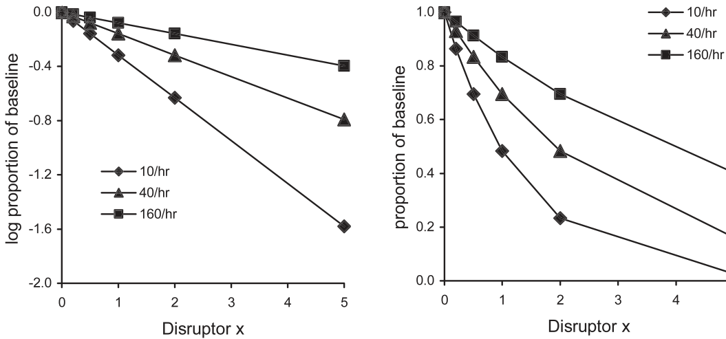
Figure 1. Simulated predictions of Equations 2 (left) and 3 (right) for the effects of a disruptor ( x ) at three values of reinforcers per hour ( r ). Note that as x increases, log proportions of baseline decrease linearly with no lower bound, whereas simple proportions decrease according to nonlinear (exponential) functions with 0 as the lower limit. Note also that for a given value of x , decreases are related inversely to the value of r .
