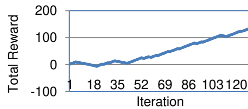
Figure 17. Total rewards of Q learning obstacle avoidance behavior.
