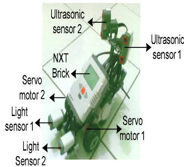
Figure 8. LEGO NXT Robot for autonomous navigation task
