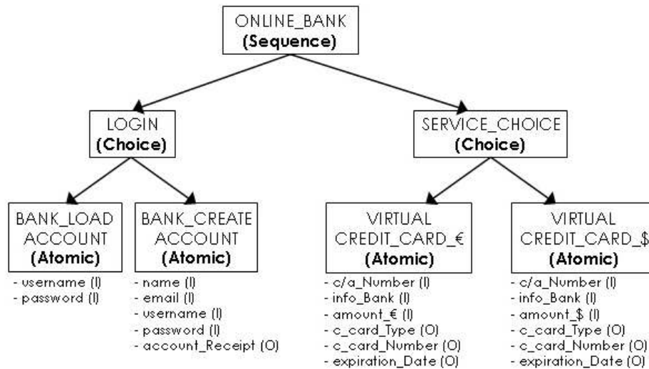
Fig. 2. Process model of Online_Bank service.
