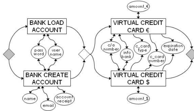
Fig. 9 Petri net representation of the Online_bank service.
