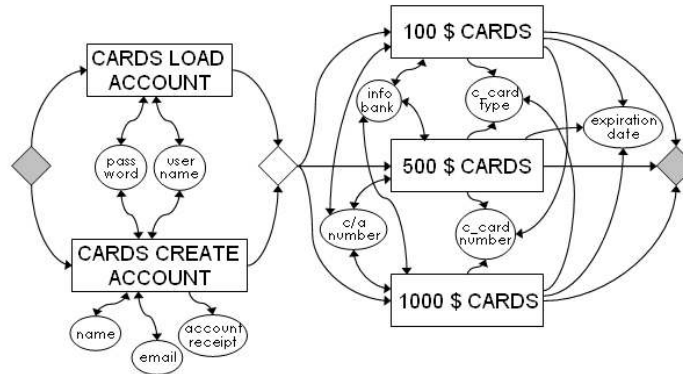
Fig. 10. Petri net representation of the Prepaid_Cards service.
