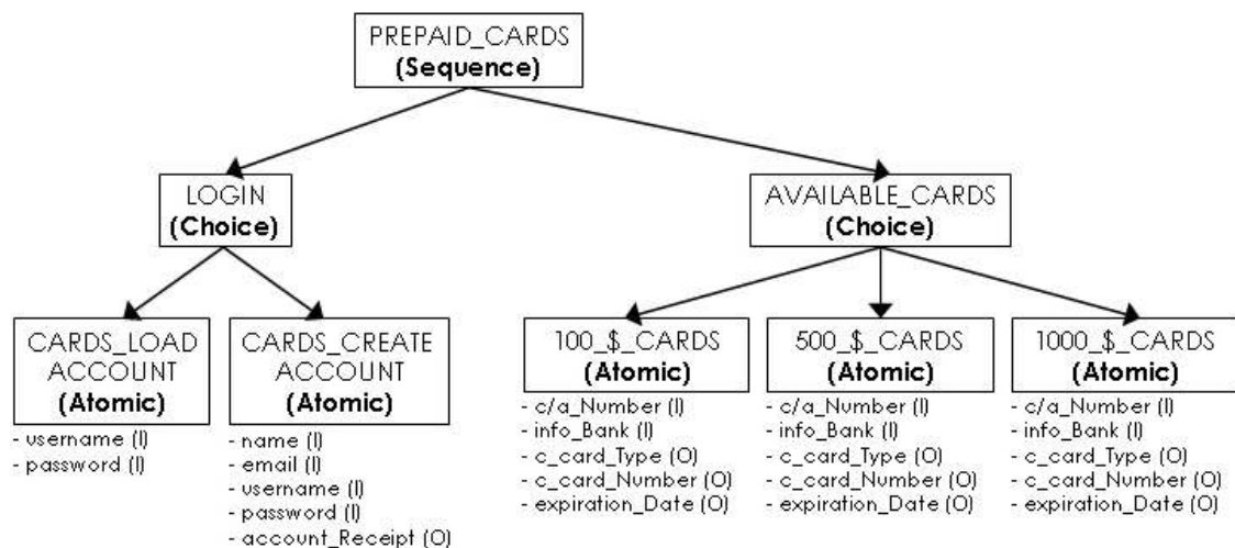
Fig. 3. Process model of Prepaid_Cards service.
