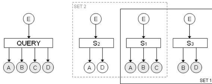
Fig. 7. Example of minimal sets of services.
