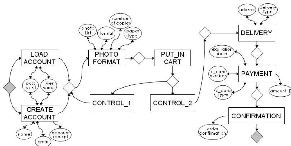
Fig. 8. Petri net representation of the Photo_Service.
