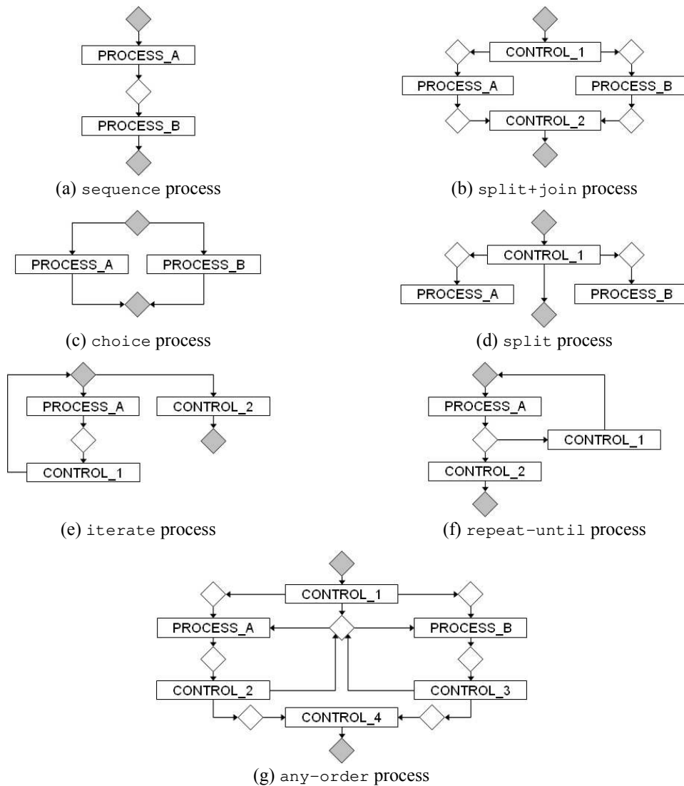
Fig. 5. Modelling OWL-S atomic processes as Petri net transitions.
