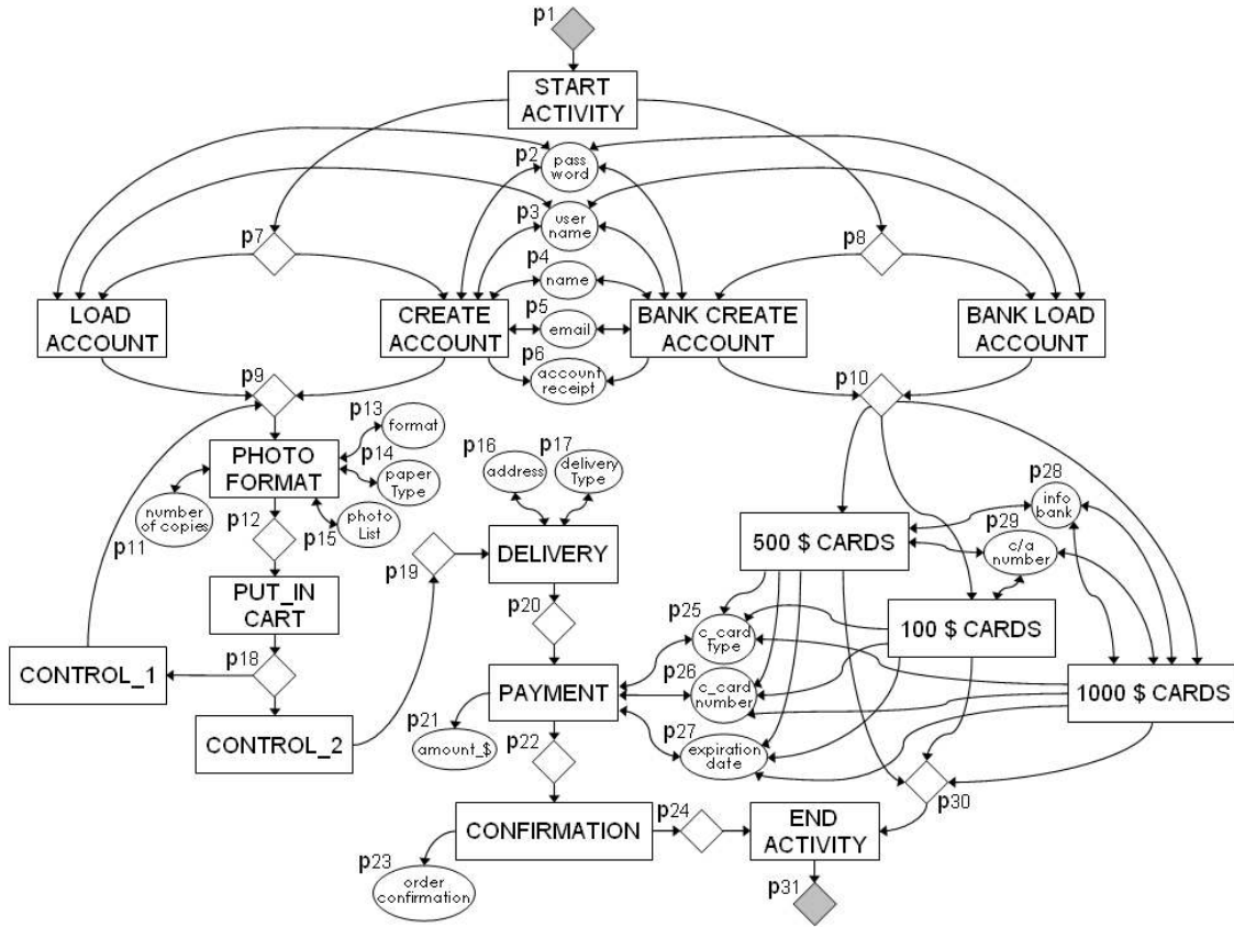
Fig. 12. The global Petri net for the second composition.
