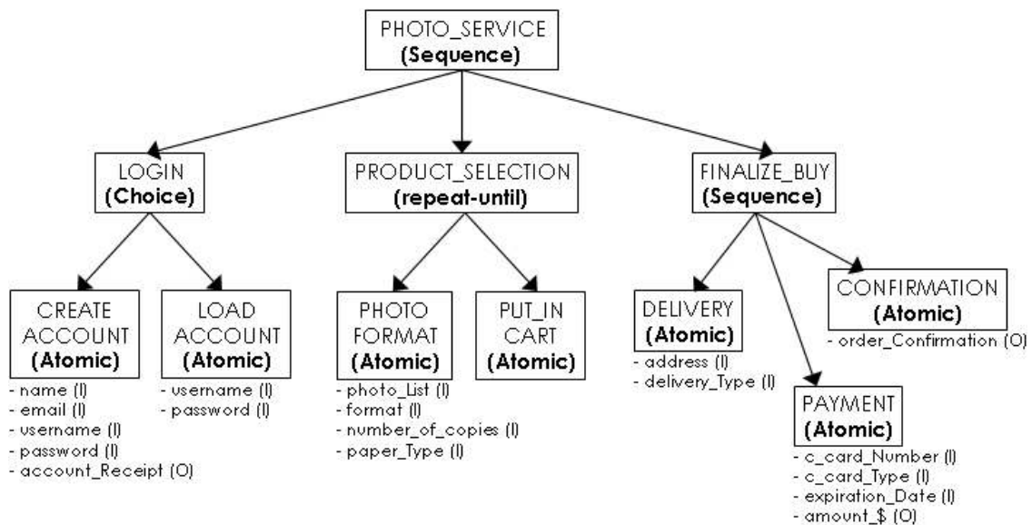
Fig. 1. Process model of Photo_service
