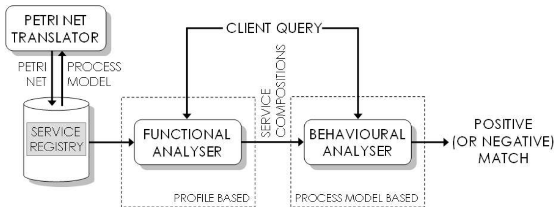
Fig. 6. Matchmaking system architecture
