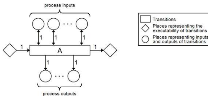
Fig. 4. Modelling OWL-S atomic processes as Petri net transitions.
