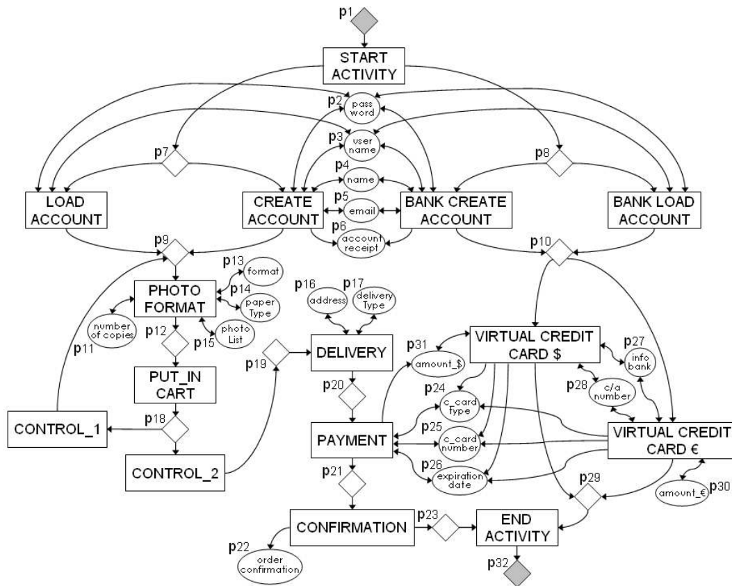
Fig. 11. The global Petri net for the first composition.
