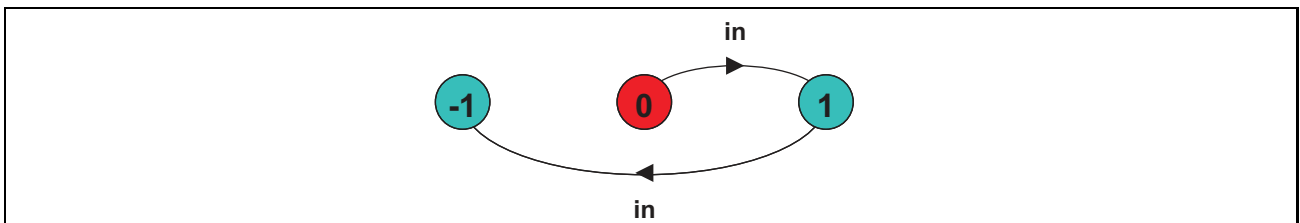
Figure 4.8: LTS model of process P2 composed with property IN_OUT.
