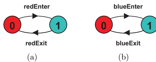
Figure 6.3: LTS models of (a) the red car and (b) the blue car.
