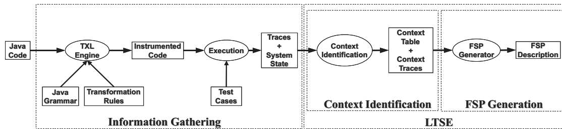
Figure 3.5: General view of the model extraction process.
