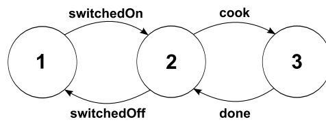
Figure 2.2: LTS of the microwave oven.
