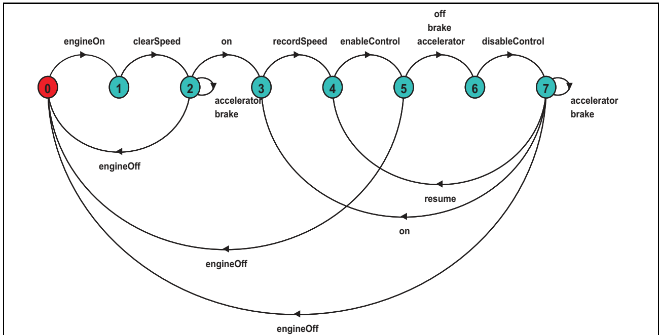
Figure B.4: LTS model of the cruise controller.
