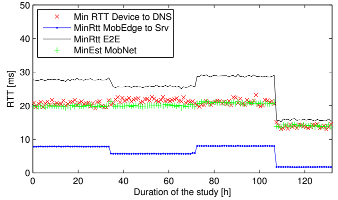
Fig. 4. Exemplary RTT measurements for one device with the estimated RTT within the mobile operator's domain
