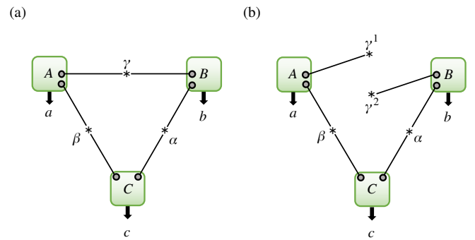
FIG. 5. Illustration of inflation in the triangle scenario. (a) is the triangle network, formed by three parties and three bipartite sources. By measuring the systems that are sent from their respective sources, the parties produce outcomes a , b and c according to the probability distribution P_{\text{obs}}^{\text{ABC}} . (b) A possible inflation considers two copies of the source \gamma . One sends a system only to Alice, and the other one sends a system only to Bob. By measuring their respective systems the parties produce outcomes according to the distribution P_{\text{inf}}^{\text{ABC}} . In both cases, Alice and Charlie receive the same systems from the same type of sources, so P_{\text{obs}}^{\text{AC}} = P_{\text{inf}}^{\text{AC}} . This is not the case for Alice and Bob, since P_{\text{inf}}^{\text{AB}} = P_{\text{inf}}^{\text{A}} P_{\text{inf}}^{\text{B}} (which also equates to P_{\text{obs}}^{\text{A}} P_{\text{obs}}^{\text{B}} ), while P_{\text{obs}}^{\text{AB}} \neq P_{\text{obs}}^{\text{A}} P_{\text{obs}}^{\text{B}} in general.
