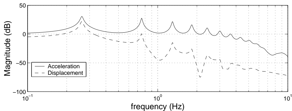
(c) 20-Story Building Model
