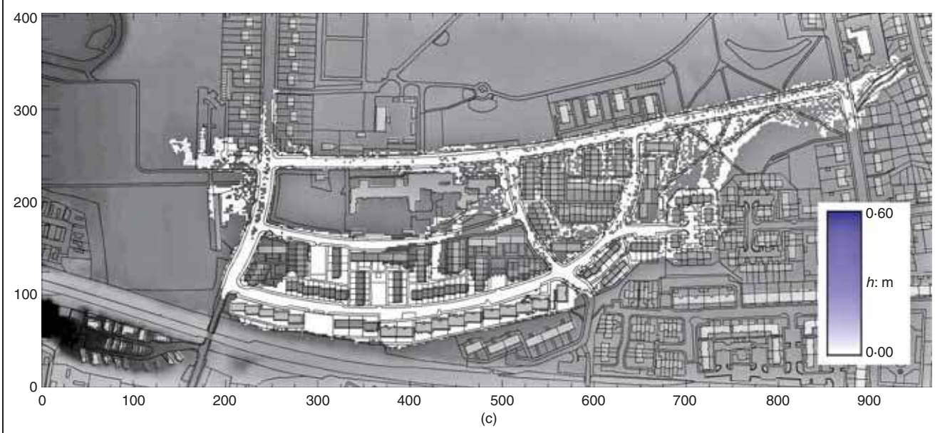
Fig. 7. Magnitude of range in water depth ( h ) predicted by each model at 60 minutes into the event for the ensemble of varying friction coefficient simulations shown in Table 2: (a) DIVAST; (b) DIVAST-TD; (c) JFLOW; (d) LISFLOOD; (e) TRENT; and (f) TUFLOW
