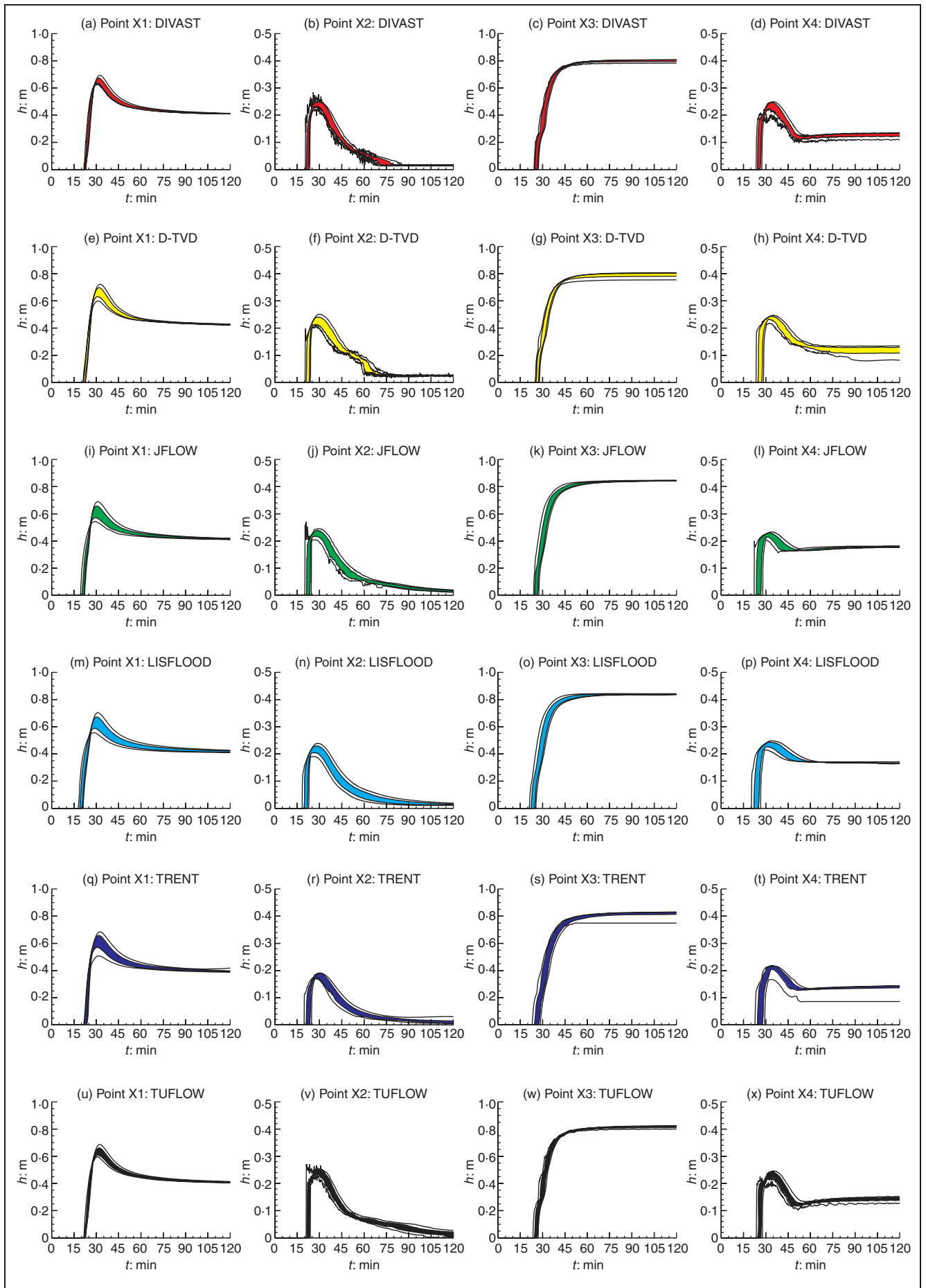
Fig. 5. Cumulative distribution functions of water depth predicted by each model at points X1–X4 on Fig. 1 for the ensemble of varying friction coefficient simulations shown in Table 2. The black lines represent the minimum and maximum water depths predicted over the ensemble, while the shaded area represents the 25–75% range of the cumulative distribution
