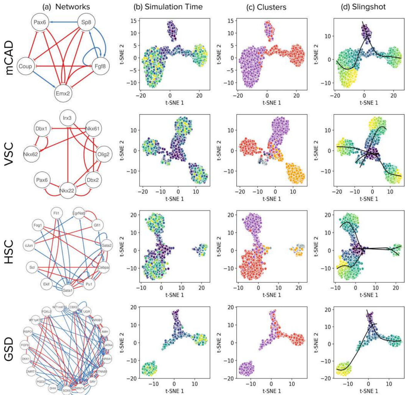
Figure 3: Visualization of t-SNE projections of simulations reveals trajectories leading to steady states that correspond to those of the curated models. Each row in the figure corresponds to a model, indicated on the left: Mammalian Cortical Area Development (mCAD), Ventral Spinal Cord Development (VSC), Hematopoietic Stem Cell Differentiation (HSC), and Gonadal Sex Determination (GSD). (a) Network diagrams of the models. (b) t-SNE visualizations of 2,000 cells sampled from BoolODE output. The color of each point indicates the corresponding simulation time. (c) Each color corresponds to a different subset of cells obtained by using k -means clustering of simulations, with k set to the number of
