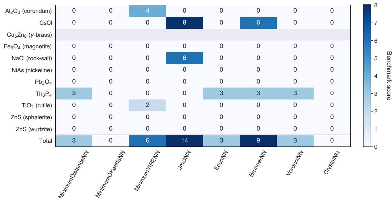
Figure S12: Ability of near neighbor algorithms ( x -axis) to reproduce literature descriptions of anion coordination for the binary structures in the MaterialsCoord benchmark suite ( y -axis). Scores are color-coded, with darker colors indicating greater deviation from the literature coordination number. The total score for each algorithm is calculated as the sum of the scores across all structures.
