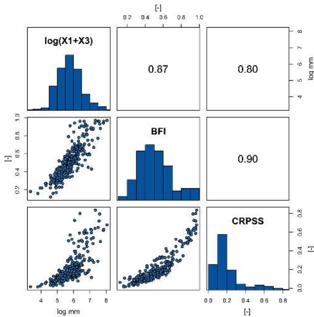
Figure 8. Scatterplot matrix between catchment storage capacity (X1 soil moisture store capacity [mm] + X3 groundwater store capacity [mm]), BFI, and ESP skill (CRPSS) with n = 314 using the non-parametric Spearman's rank correlation coefficient \rho . Skill is the 1-month CRPSS skill score magnitude averaged across all 12 initialization months. Catchment storage capacity (X1 + X3) was re-expressed by taking the natural log, as raw values are heavily positively skewed.
