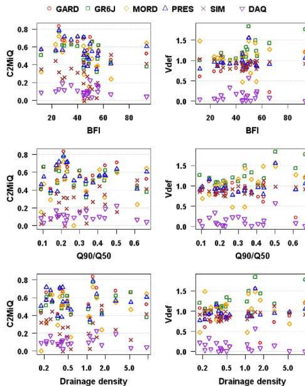
Figure 7. Relation between mean performance in simulation on the two validation periods in terms of C2M_i (left panel) and Vdef (right panel), and catchment or streamflow characteristics (top panels: base-flow index; middle panels: Q_{90}/Q_{50} ratio; bottom panels: drainage density) for the 21 catchments and the models tested.
