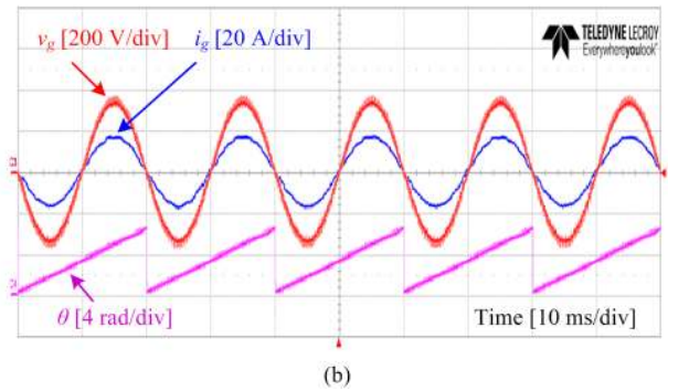
Fig. 12. Performance of the two-stage single-phase grid-connected PV system: (a) the PV power extraction during the MPPT operation, and (b) the grid voltage v_g , grid current i_g and the phase angle \theta during the steady-state MPPT operation (3 kW).
