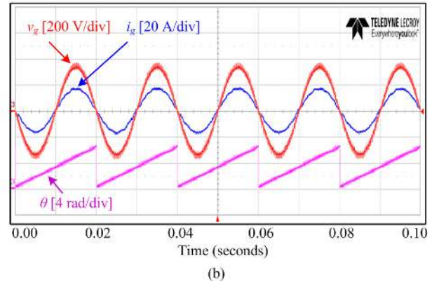
Fig. 12. Performance of the two-stage single-phase grid-connected PV system: (a) the PV power extraction during the MPPT operation, and (b) the grid voltage v_g , grid current i_g and the phase angle \theta during the steady-state MPPT operation (3 kW).
