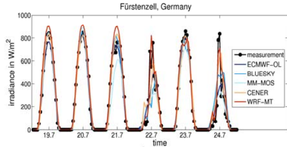
Figure 4: Measured irradiance in comparison to predicted irradiances for six days in July 2007 for the station Fürstzell.
