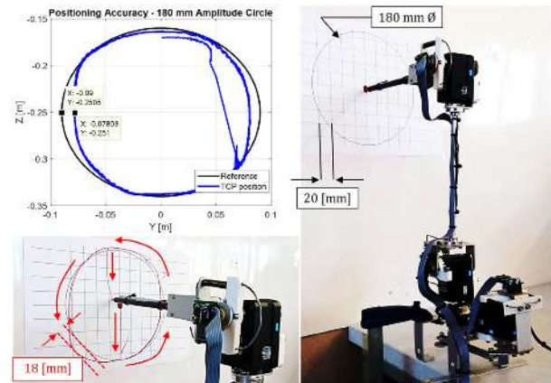
Fig. 9. Evaluation of the positioning accuracy drawing an 18 cm \emptyset circle.
