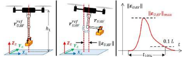
Fig. 6. Benchmark for evaluating the performance of the multirotor position controller affected by the dynamic coupling with the manipulator.
