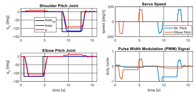
Fig. 11. Joint variables (left), servo speed and PWM (right) of the shoulder pitch and elbow pitch joints during the lift load experiment.
