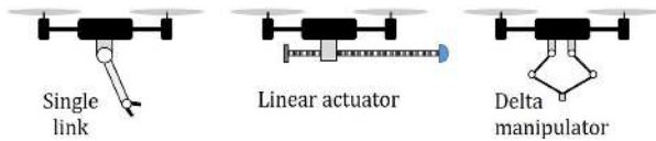
Fig. 7. Three different morphologies of aerial manipulators.
