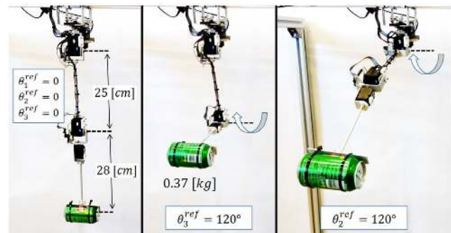
Fig. 10. Execution of the lift load benchmark with a 33 ml can (370 g).
