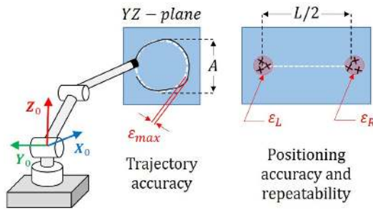
Fig. 1. Benchmarks for evaluating the accuracy and repeatability of the manipulator. A pen attached to the end effector is used to draw a circle and the marks, compared with respect to a reference pattern printed on a panel.
