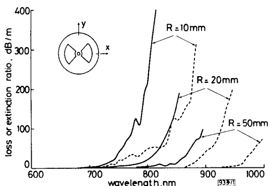
Fig. 1 Spectral polarisation extinction-ratio (solid lines) for a single loop of bend radius shown
